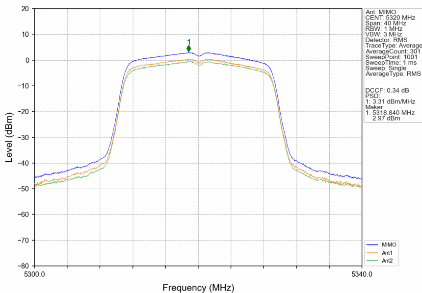
802.11ac(VHT20)_HCH_5320MHz_MIMO_NTNV
