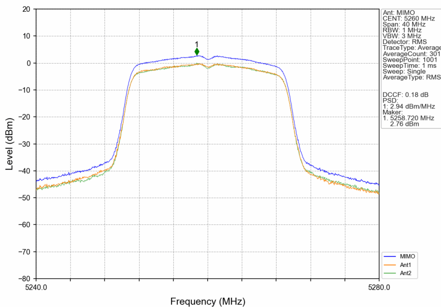
802.11n(HT20)_LCH_5260MHz_MIMO_NTNV
