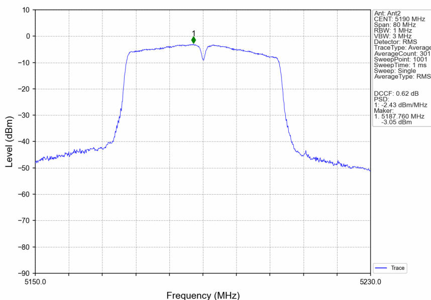
802.11ac(VHT40)_LCH_5190MHz_MIMO_NTNV
