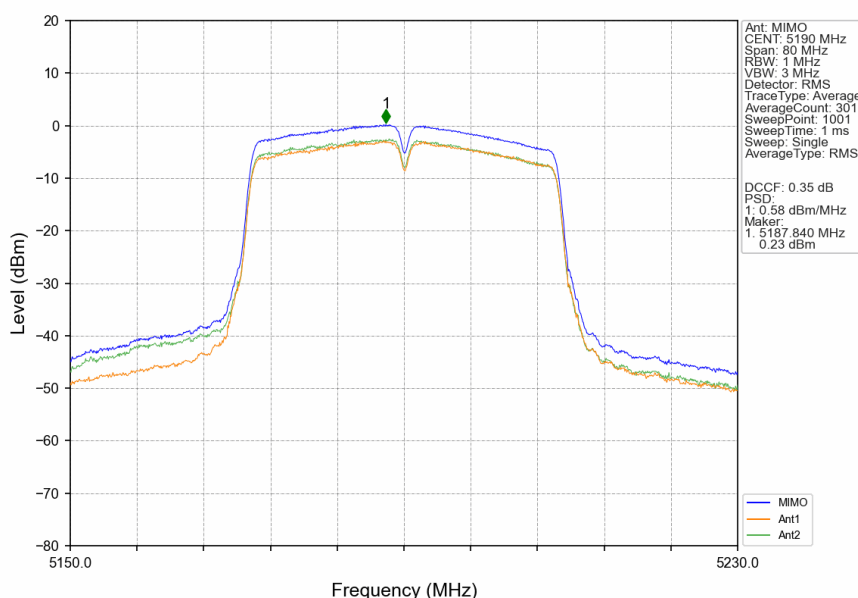
802.11n(HT40)_LCH_5190MHz_MIMO_NTNV
