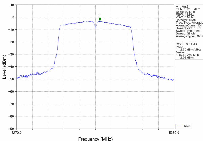
802.11ac(VHT40)_HCH_5310MHz_Ant2_NTNV
