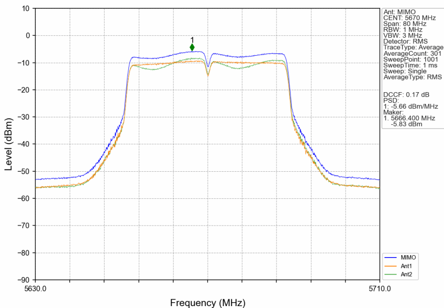
802.11n(HT40)_HCH_5670MHz_MIMO_NTNV
