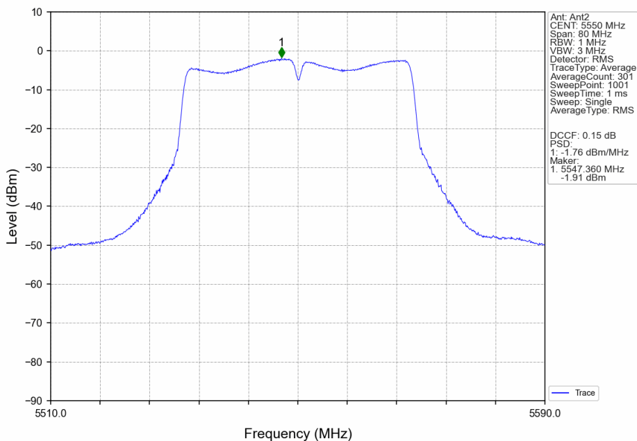
802.11n(HT40)_MCH_5550MHz_Ant2_NTNV
