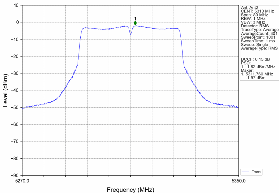
802.11n(HT40)_HCH_5310MHz_Ant2_NTNV
