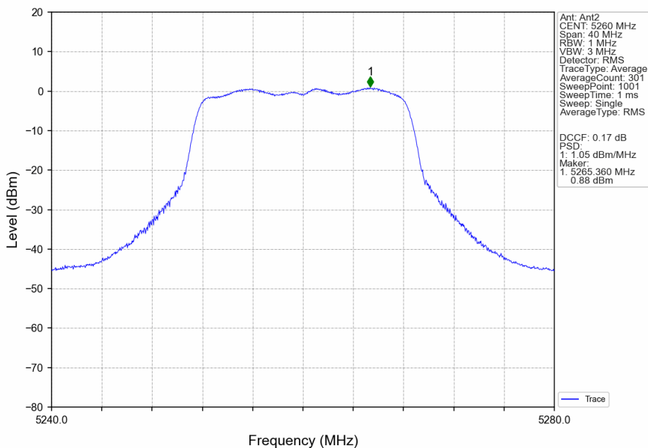
802.11a_LCH_5260MHz_Ant2_NTNV
