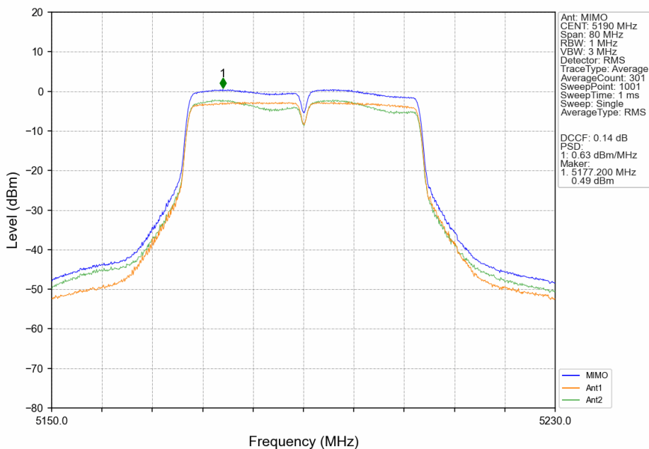
802.11ac(VHT40)_LCH_5190MHz_MIMO_NTNV
