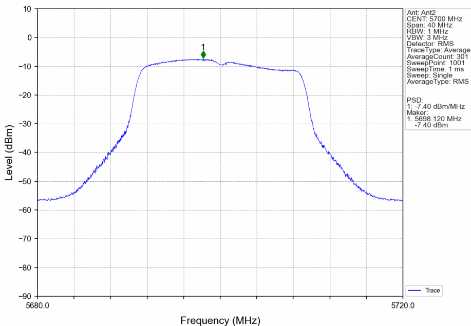
802.11ac(VHT20)_HCH_5700MHz_Ant2_NTNV
