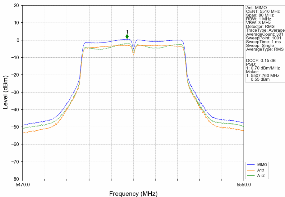
802.11n(HT40)_LCH_5510MHz_MIMO_NTNV
