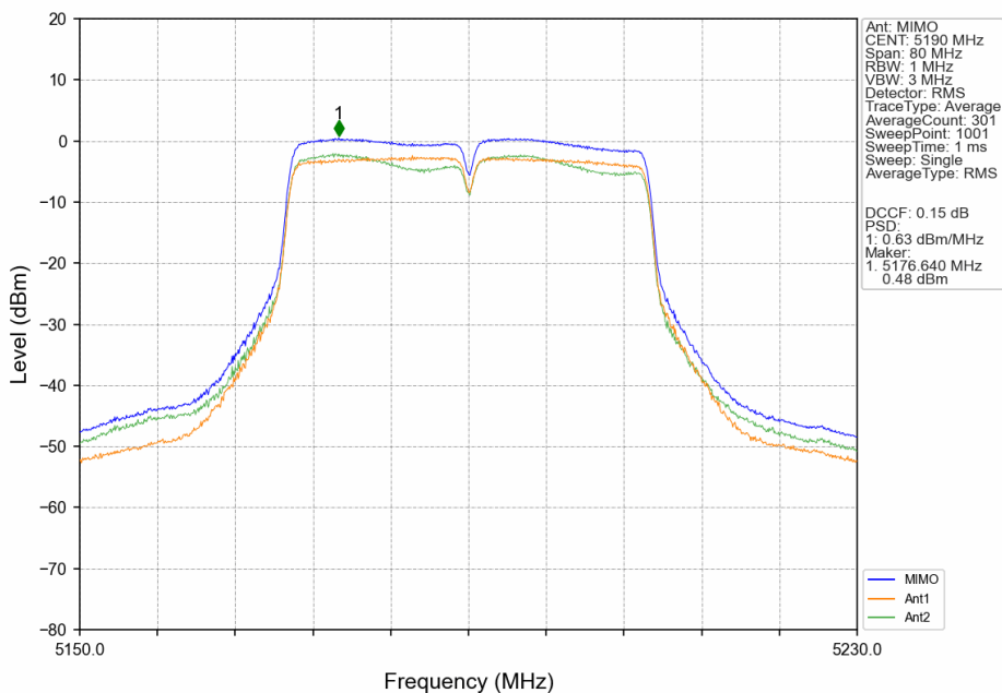
802.11n(HT40)_LCH_5190MHz_MIMO_NTNV
