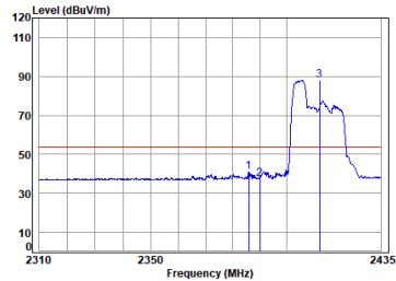
11ax_20M_Partial_RU52_TX_CH_01_Vertical-Avg
