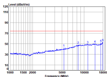
11n_HT(40M)_TX_CH_03_Horizontal-Peak
