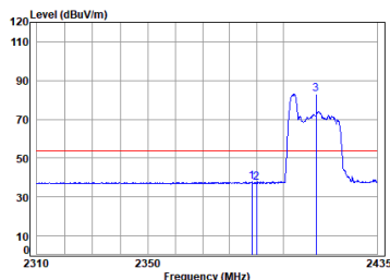
11ax_20M_Partial_RU26_TX_CH_01_Horizontal-Avg
