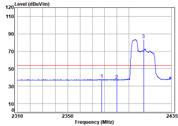
11ax_20M_Partial_RU52_TX_CH_01_Horizontal-Avg
