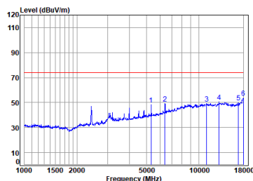
11n_HT(40M)_TX_CH_03_Vertical-Peak
