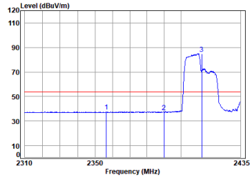
11ax_20M_Partial_RU106_TX_CH_01_Horizontal-Avg
