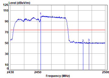
11ax_40M_Partial_RU242_TX_CH_09_Vertical-Peak
