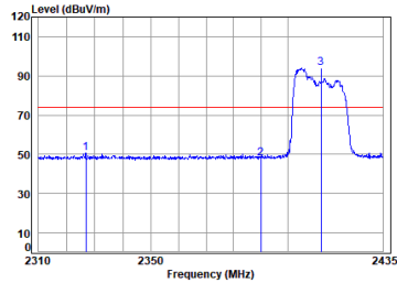
11ax_20M_Partial_RU52_TX_CH_01_Horizontal-Peak
