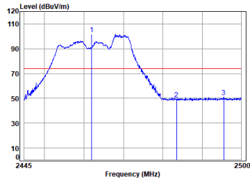
11ax_20M_Partial_RU52_TX_CH_11_Vertical-Peak
