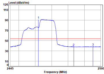
11ax_20M_Partial_RU106_TX_CH_11_Vertical-Avg
