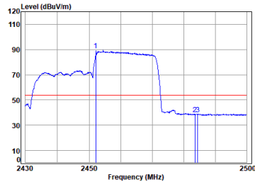
11ax_40M_Partial_RU242_TX_CH_09_Vertical-Avg
