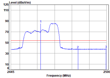
11ax_20M_Partial_RU52_TX_CH_11_Horizontal-Avg
