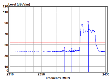
11ax_20M_Partial_RU26_TX_CH_01_Vertical-Avg
