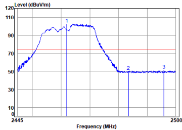
11ax_20M_Partial_RU106_TX_CH_11_Vertical-Peak
