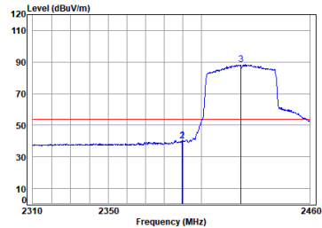
11ax_40M_TX_CH_03_Vertical-Avg
