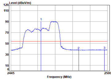
11ax_20M_Partial_RU52_TX_CH_11_Vertical-Avg
