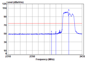
11ax_20M_Partial_RU106_TX_CH_01_Vertical-Peak
