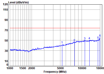
11ax_40M_TX_CH_06_Horizontal-Peak
