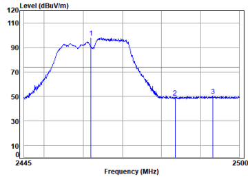
11ax_20M_Partial_RU106_TX_CH_11_Horizontal-Peak
