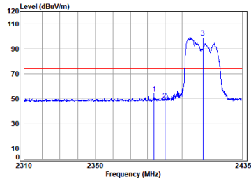
11ax_20M_Partial_RU52_TX_CH_01_Vertical-Peak
