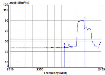
11ax_20M_Partial_RU106_TX_CH_01_Vertical-Avg
