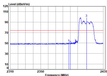
11ax_20M_Partial_RU26_TX_CH_01_Vertical-Peak
