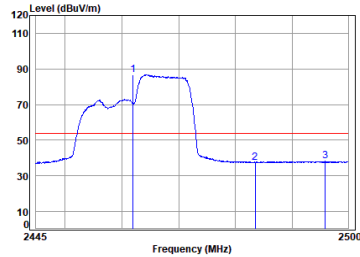
11ax_20M_Partial_RU106_TX_CH_11_Horizontal-Avg
