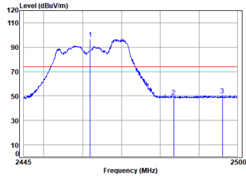
11ax_20M_Partial_RU52_TX_CH_11_Horizontal-Peak
