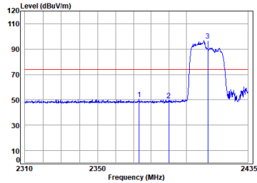
11ax_20M_Partial_RU106_TX_CH_01_Horizontal-Peak
