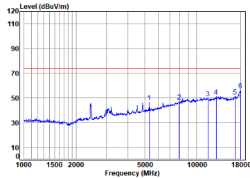
11ax_40M_TX_CH_06_Vertical-Peak
