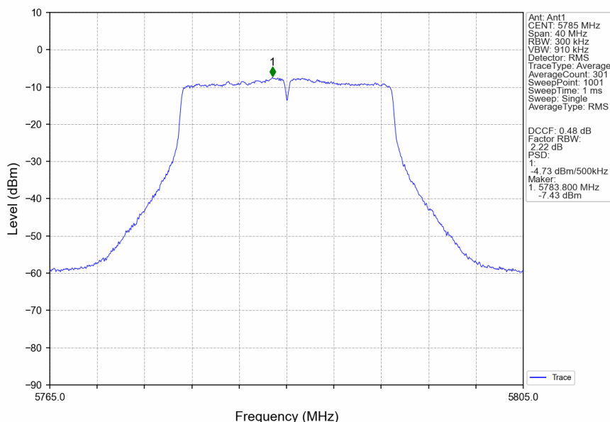
802.11ax(HEW20)_MCH_5785MHz_RU242_Left_Ant1_NTNV
