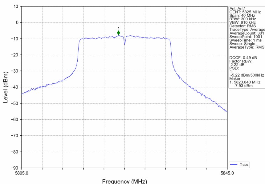
802.11ax(HEW20)_HCH_5825MHz_RU242_Left_Ant1_NTNV
