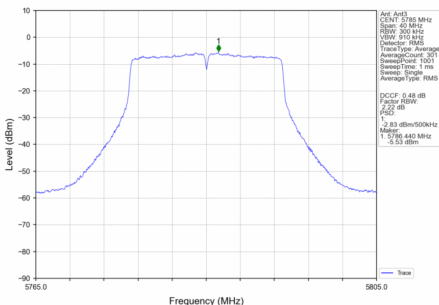
802.11ax(HEW20)_MCH_5785MHz_RU242_Left_Ant3_NTNV
