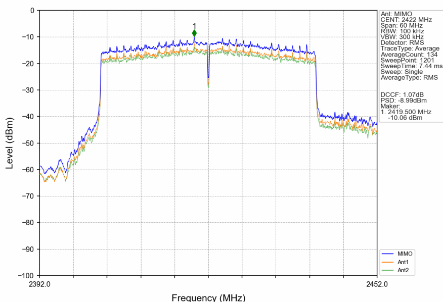
802.11ax(HEW40)_LCH_2422MHz_SU_/_MIMO_NTNV
