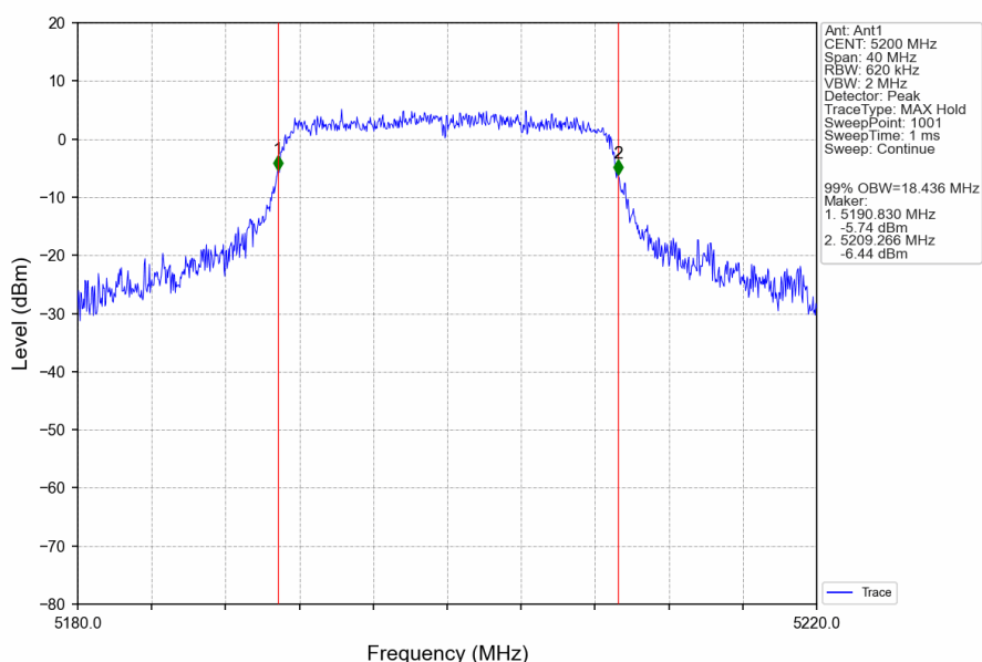
802.11n(HT20)_MCH_5200MHz_Ant1_NTNV
