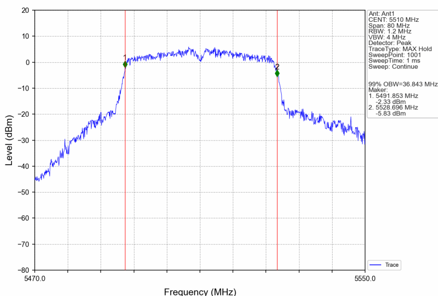
802.11ac(VHT40)_LCH_5510MHz_Ant1_NTNV
