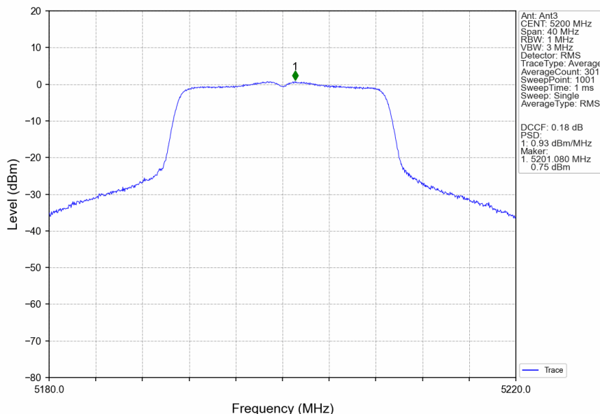
802.11n(HT20)_MCH_5200MHz_Ant3_NTNV
