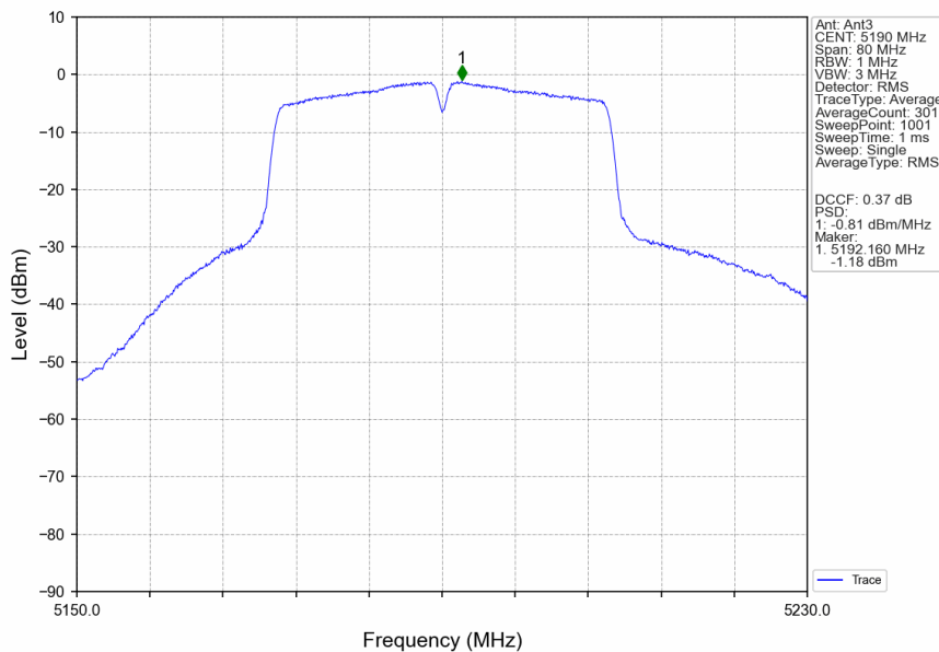
802.11n(HT40)_LCH_5190MHz_Ant3_NTNV
