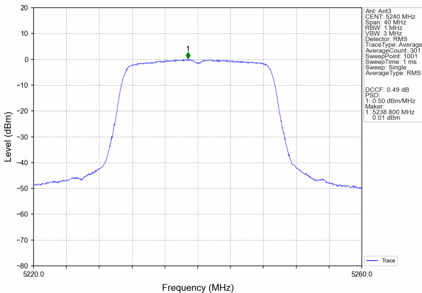
802.11ac(VHT20)_HCH_5240MHz_Ant3_NTNV
