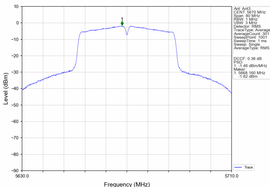
802.11n(HT40)_HCH_5670MHz_Ant3_NTNV
