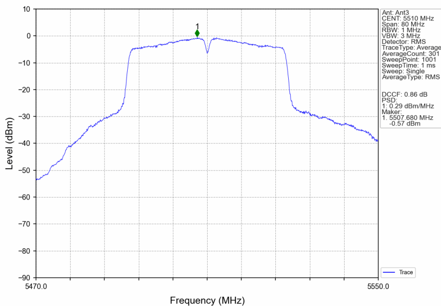
802.11ac(VHT40)_LCH_5510MHz_Ant3_NTNV
