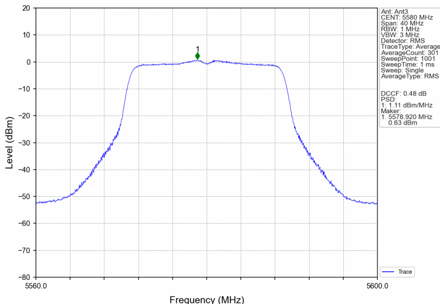
802.11ac(VHT20)_MCH_5580MHz_Ant3_NTNV
