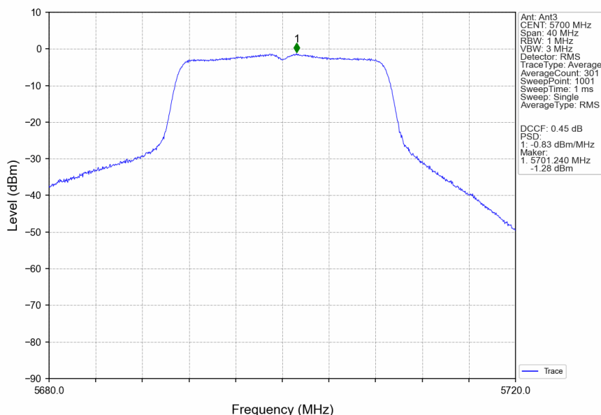
802.11ac(VHT20)_HCH_5700MHz_Ant3_NTNV
