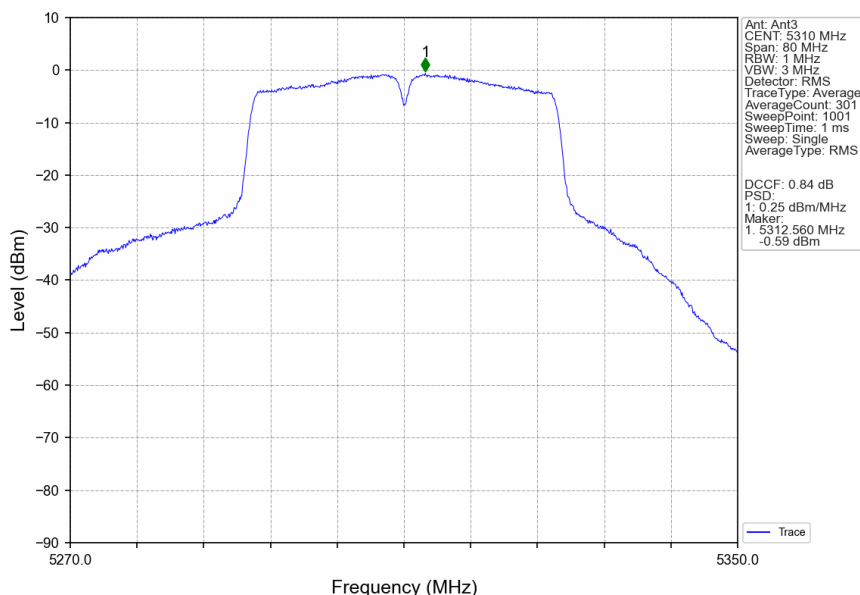
802.11ac(VHT40)_HCH_5310MHz_Ant3_NTNV
