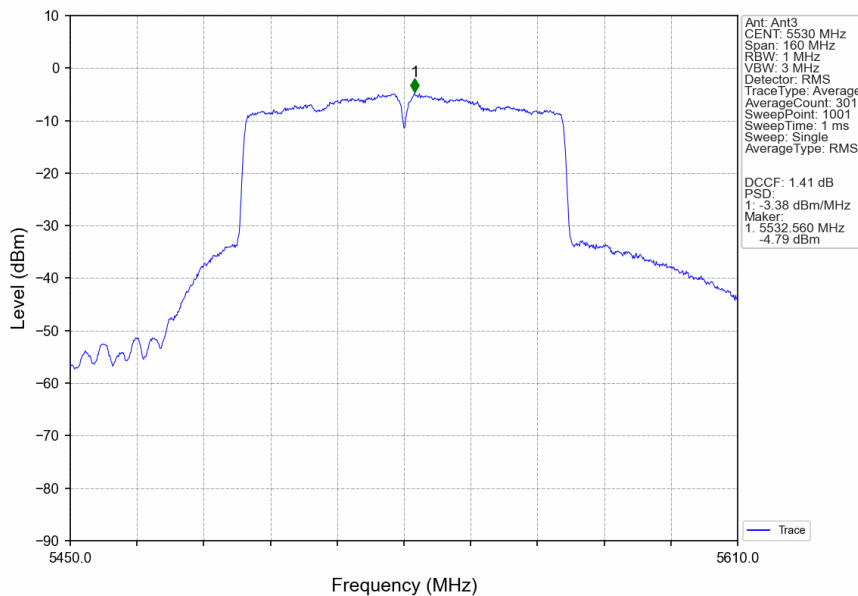
802.11ac(VHT80)_LCH_5530MHz_Ant3_NTNV
