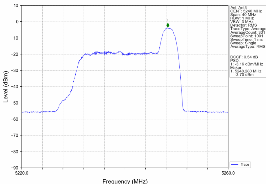
802.11ax(HEW20)_HCH_5240MHz_RU26_Right_Ant3_NTNV
