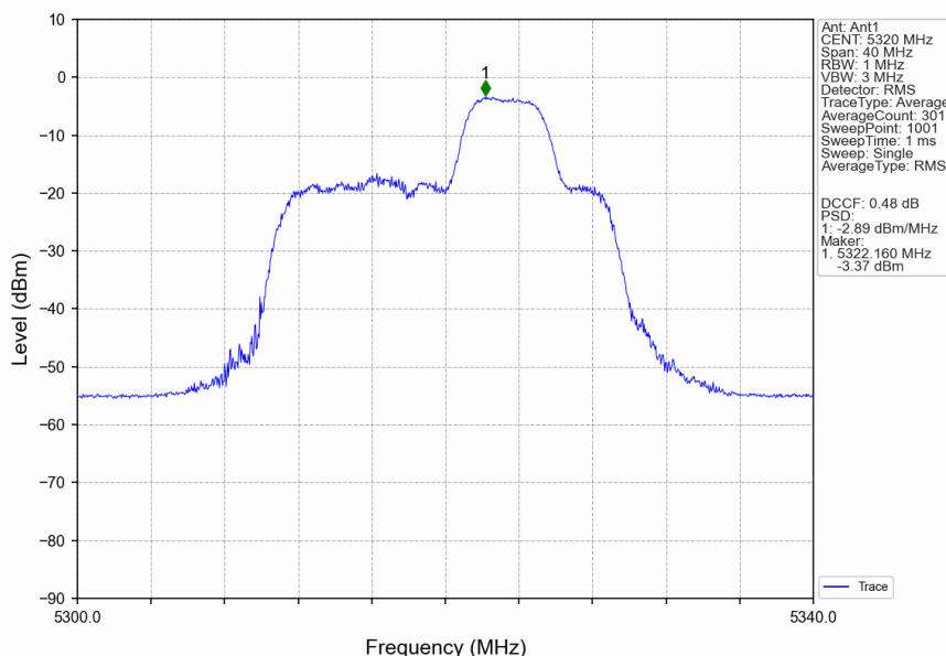
802.11ax(HEW20)_HCH_5320MHz_RU52_Right_Ant1_NTNV
