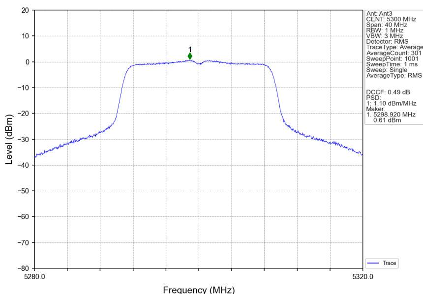
802.11ax(HEW20)_MCH_5300MHz_RU242_Left_Ant3_NTNV
