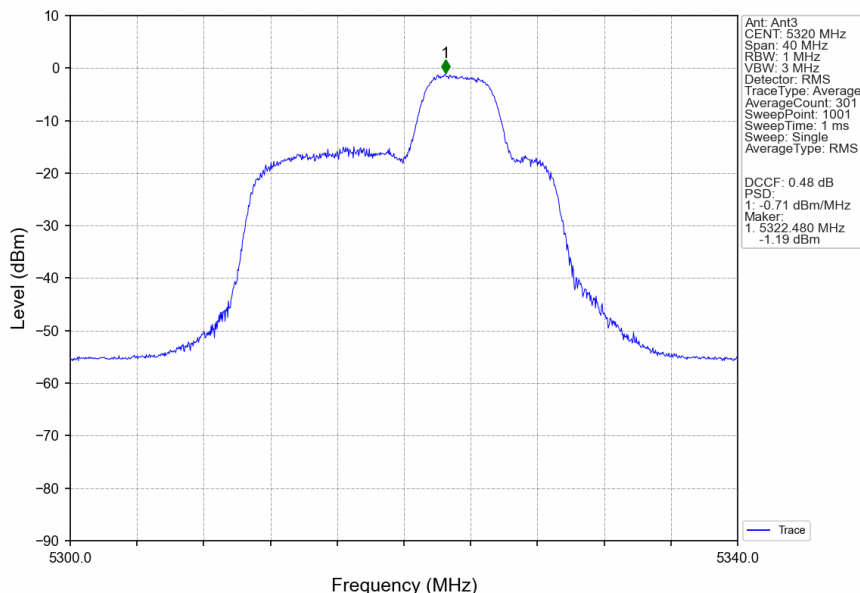
802.11ax(HEW20)_HCH_5320MHz_RU52_Right_Ant3_NTNV
