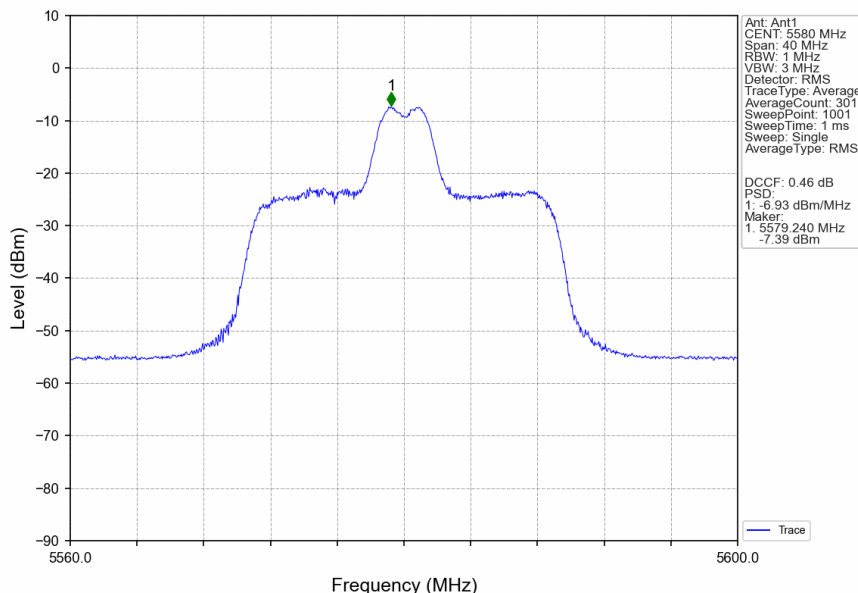
802.11ax(HEW20)_MCH_5580MHz_RU26_Mid_Ant1_NTNV
