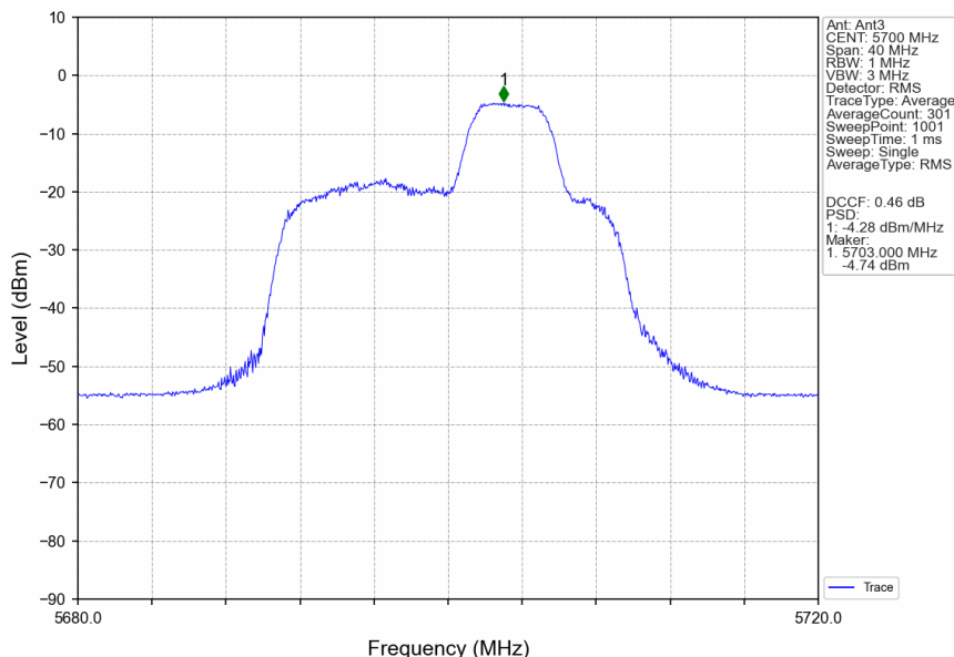
802.11ax(HEW20)_HCH_5700MHz_RU52_Right_Ant3_NTNV
