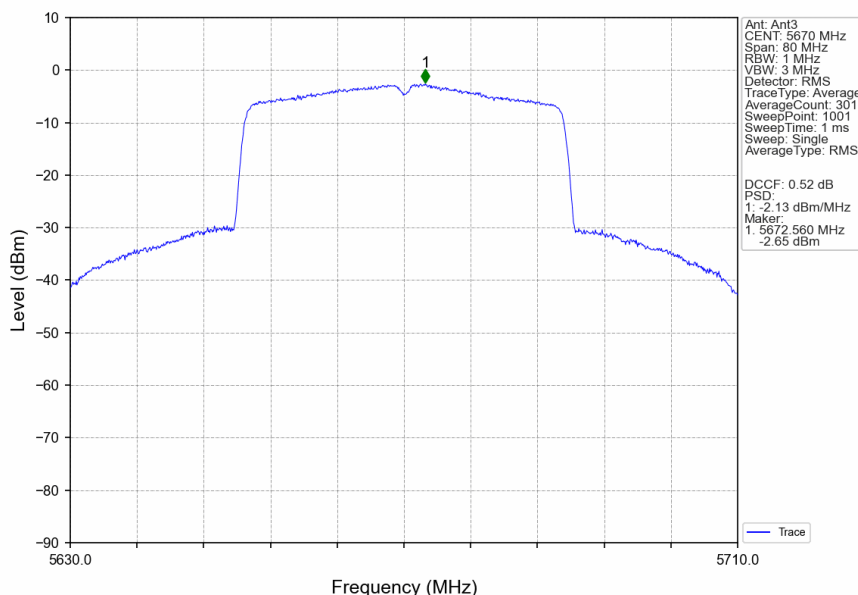
802.11ax(HEW40)_HCH_5670MHz_RU484_Left_Ant3_NTNV
