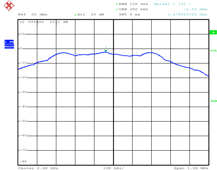
PSD 100kHz Plot on Channel 39
