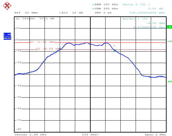
6 dB Bandwidth Plot on Channel 39
