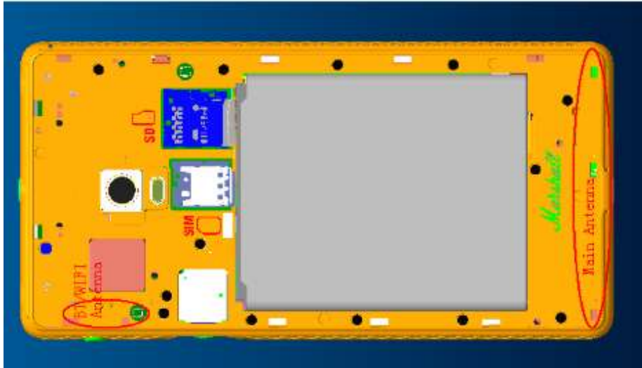
Picture of antennas
