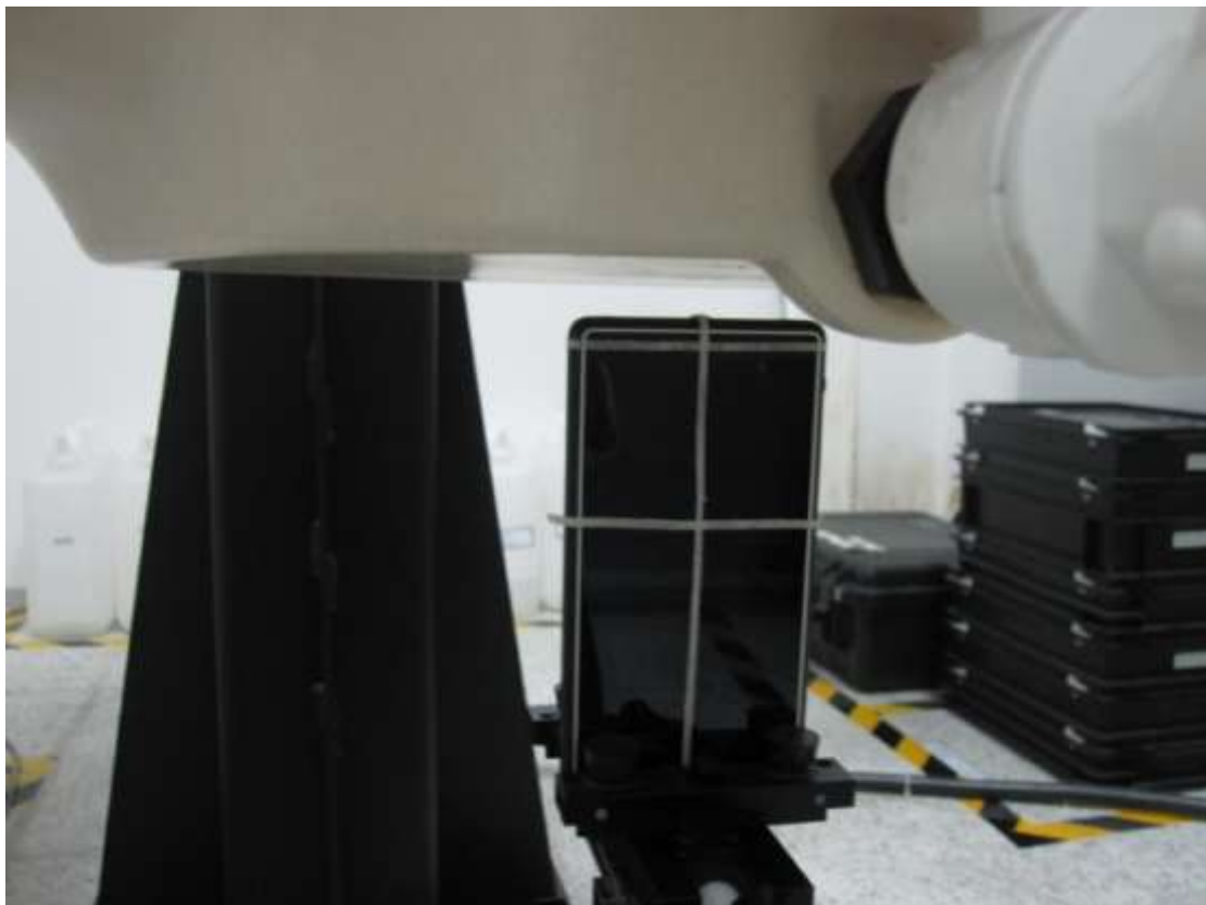
POSITION OF BODY back WITH 10mm DISTANCE
