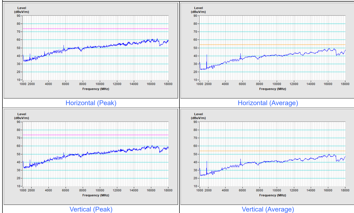
FCC 15.247 Combination 1
