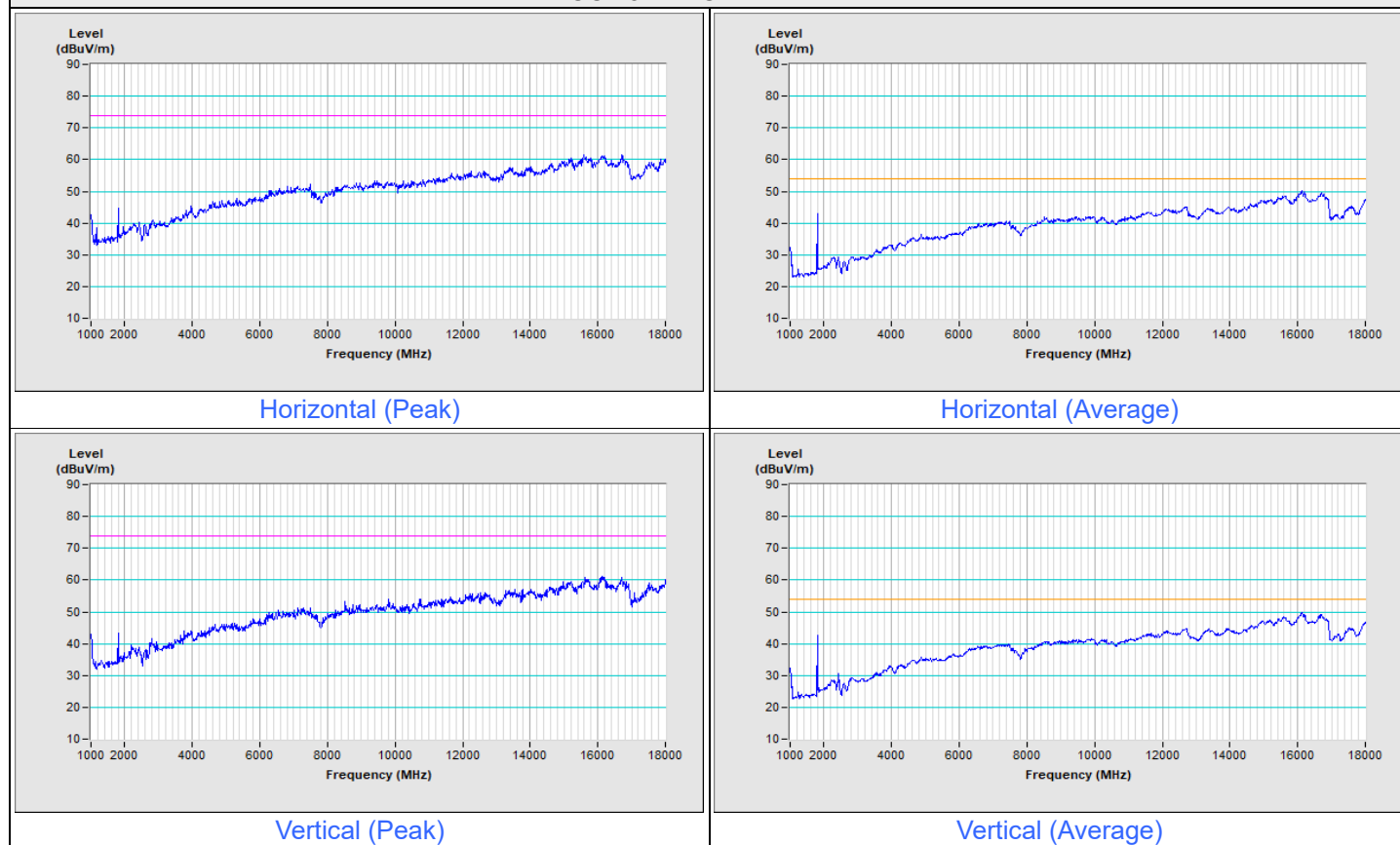
FCC 15.247 Combination 2
