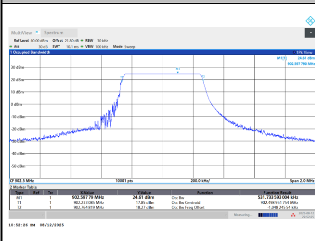
99% Occupied Bandwidth Plot on Channel 30
