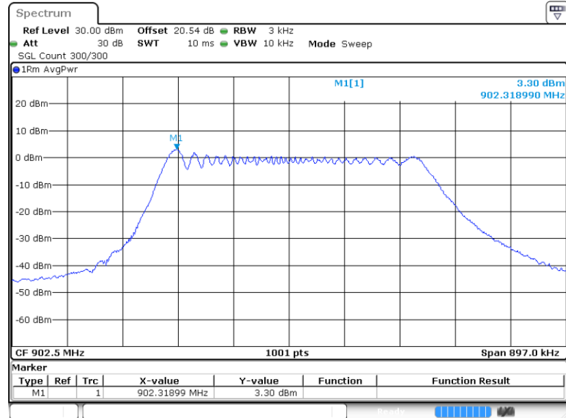
PSD 3kHz Plot on 902.5 MHz
