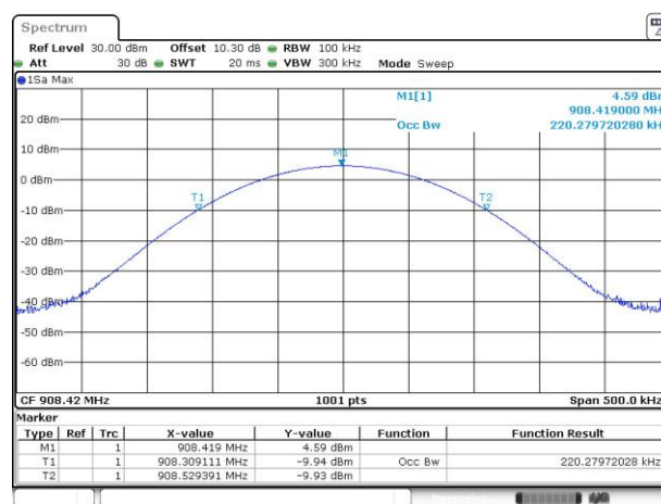
99% Bandwidth Plot on 9.6kbps
