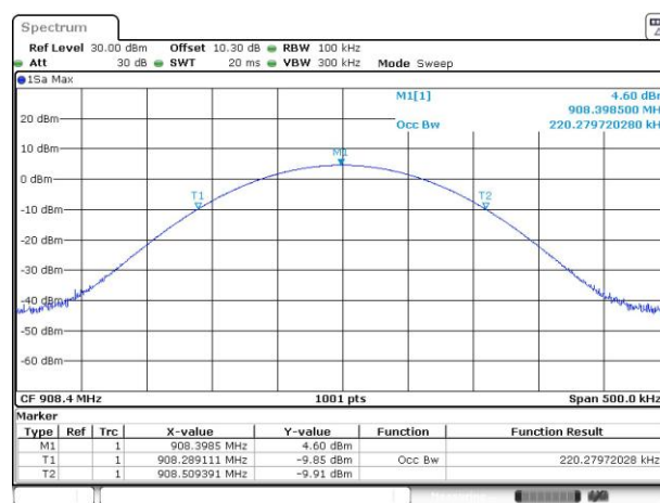
99% Bandwidth Plot on 40kbps
