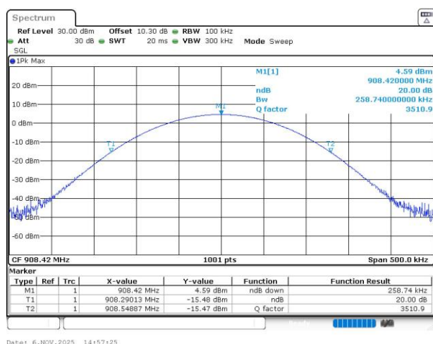
20 dB Bandwidth Plot on 9.6kbps
