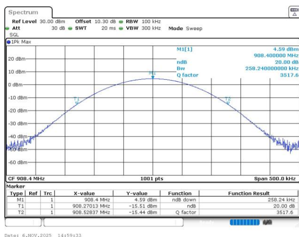
20 dB Bandwidth Plot on 40kbps
