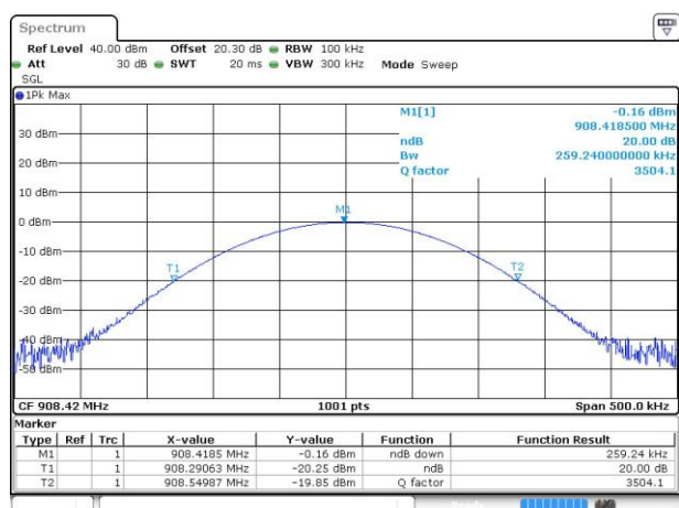
20 dB Bandwidth Plot on 9.6kbps
