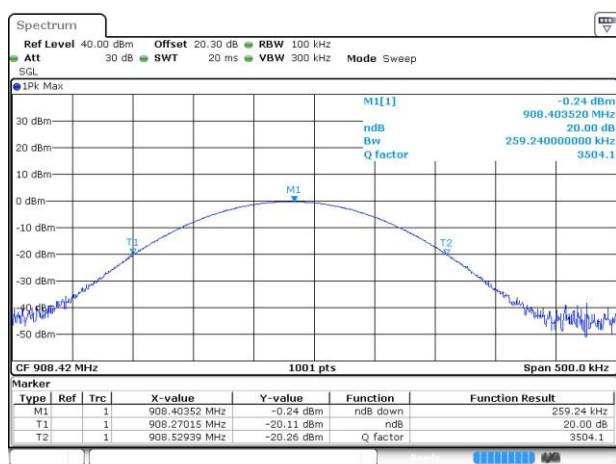
20 dB Bandwidth Plot on 40kbps
