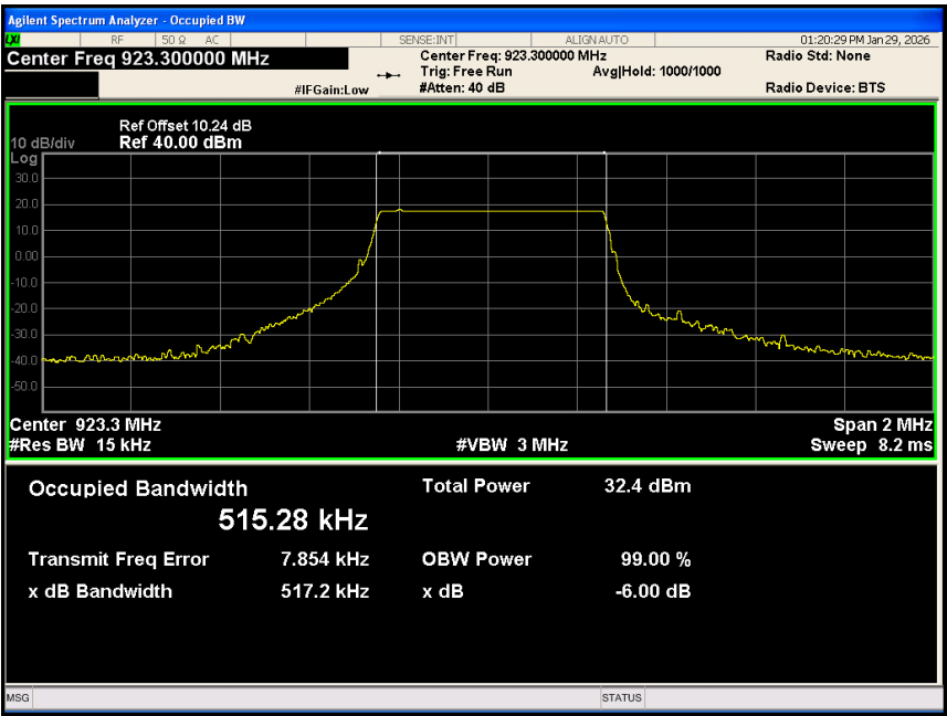
923.3MHz_Occupied Bandwidth_99 percent
