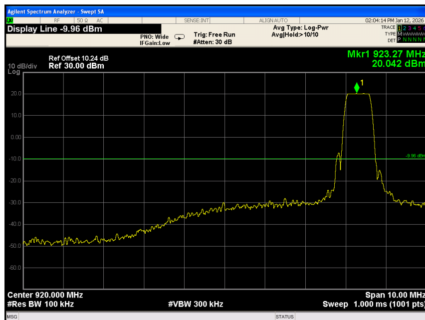
923.3MHz_ -30dBc_In Band Emissions
