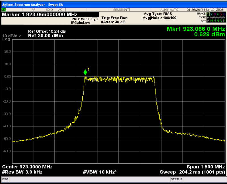
923.3MHz_ Power Spectral Density
