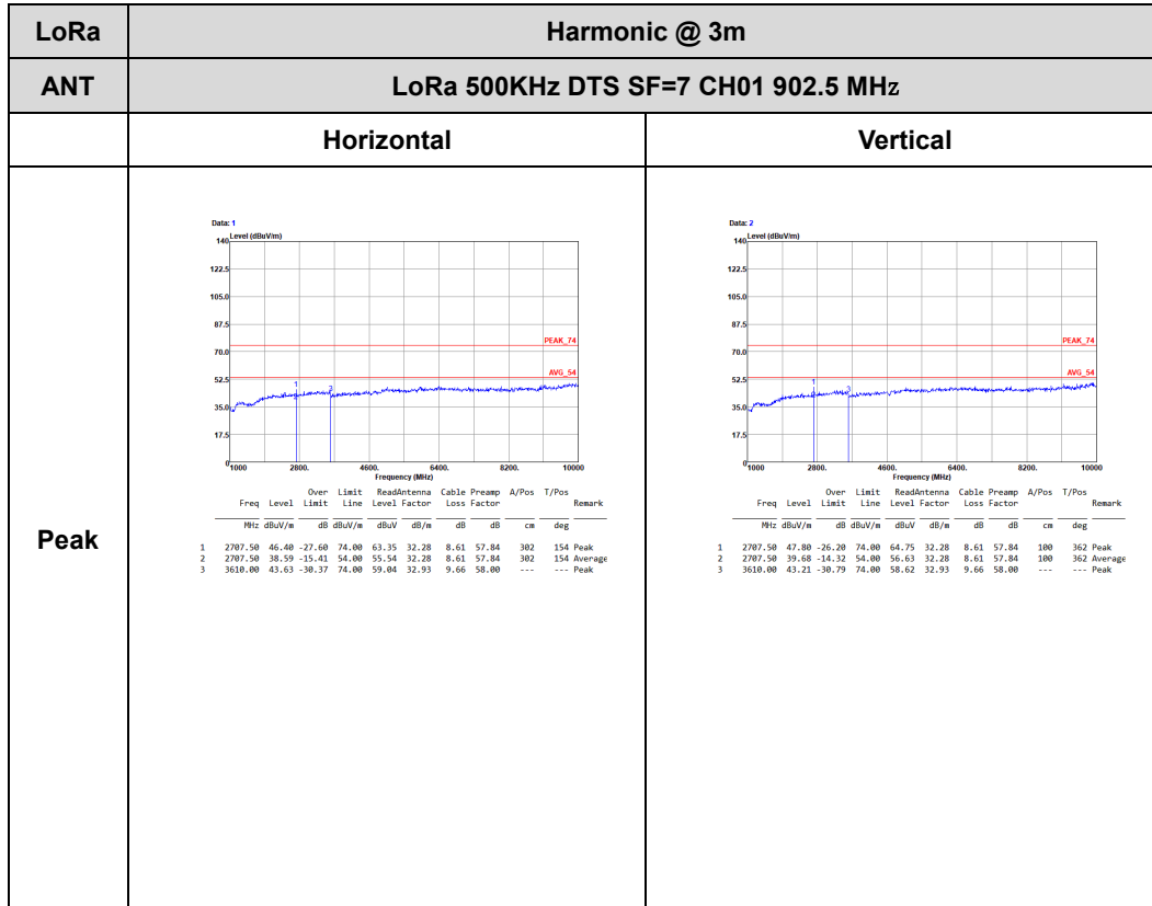
LoRa 500KHz DTS SF=7 (Harmonic @ 3m)
