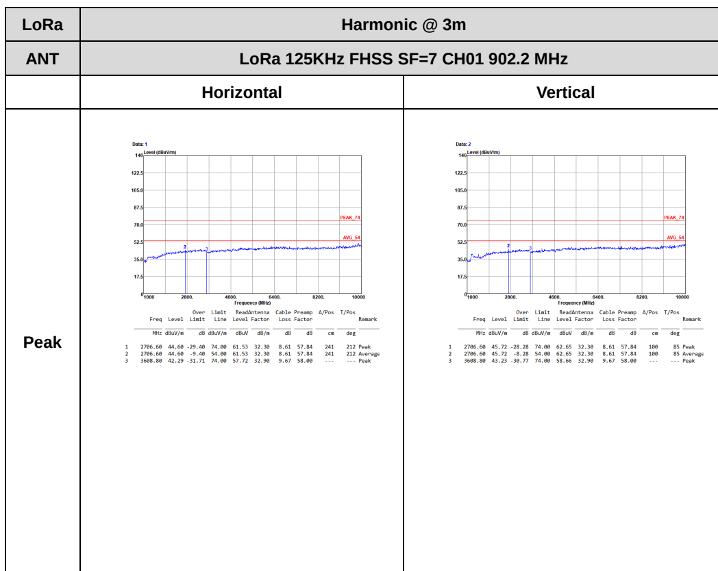
LoRa 125KHz FHSS SF=7 (Harmonic @ 3m)
