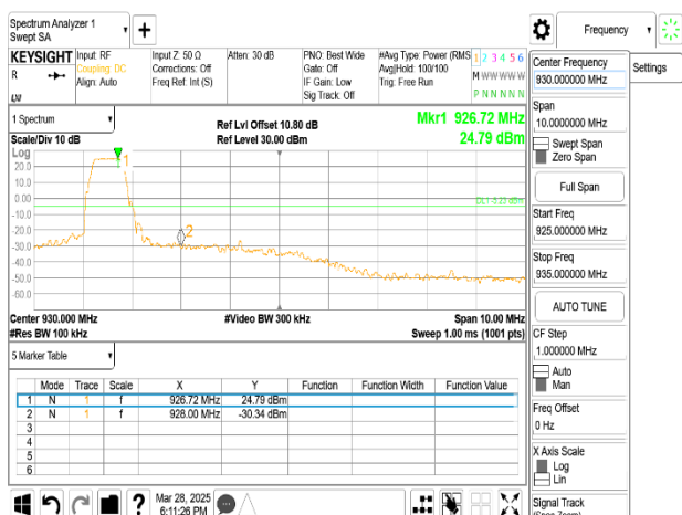
Band Edge_LoRa_SF7_HighCH-926.5MHz
