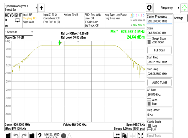
Reference Level_LoRa_SF11_HighCH-926.5MHz
