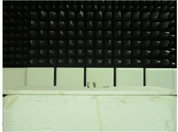
IC_RSS_247_900M_FSK_Radiated_Setup
