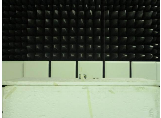
IC_RSS_247_WLAN_2.4G_Radiated_Setup
