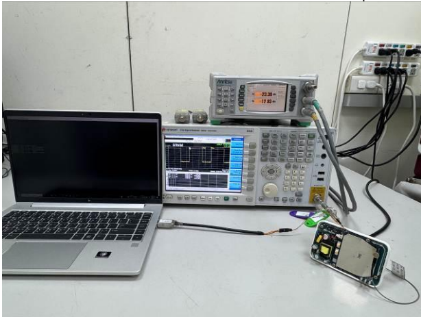
IC_RSS_247_900M_LoRa_SF7_Conducted_Setup
