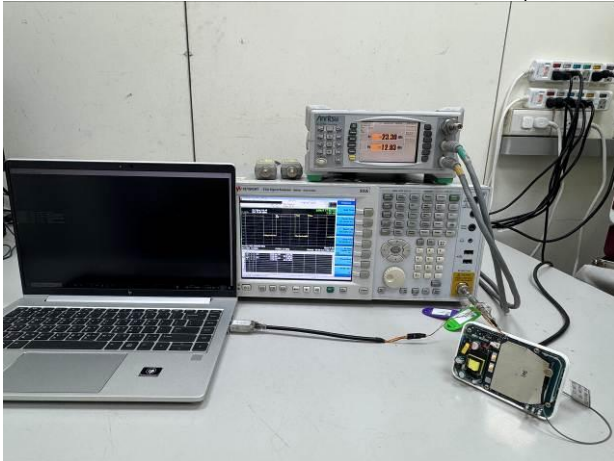
IC_RSS_247_900M_LoRa_SF7_Conducted_Setup
