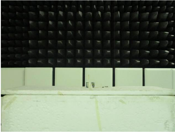
IC_RSS_247_900M_LoRa_Radiated_Setup
