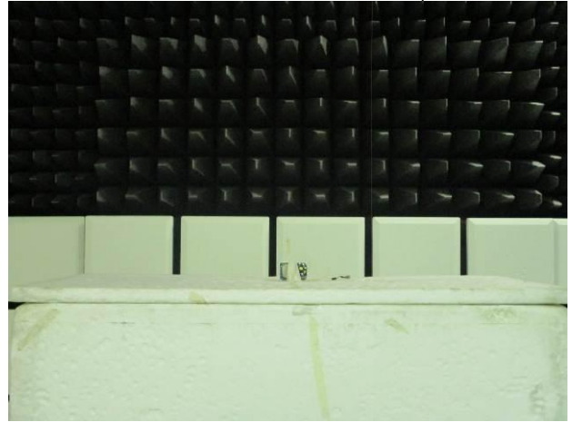
IC_RSS_247_BLE_Radiated_Setup
