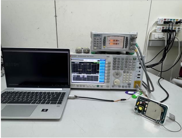
IC_RSS_247_900M_LoRa_SF11_Conducted_Setup
