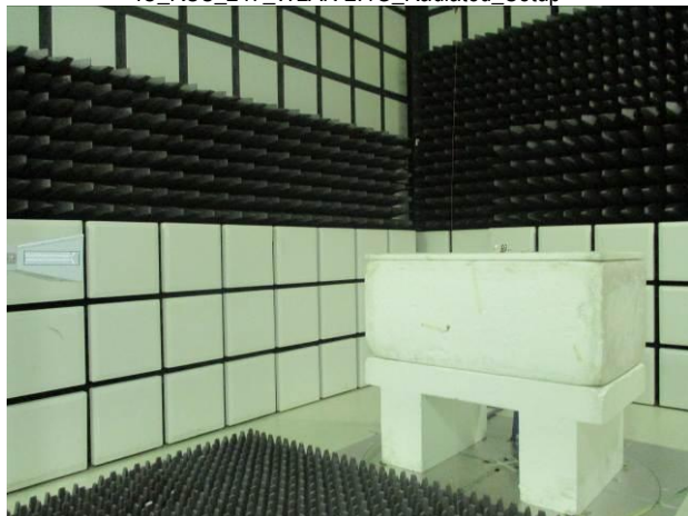
IC_RSS_247_WLAN 2.4G_Radiated_Setup
