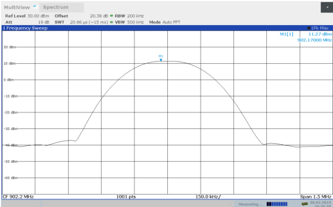
Figure 8.6-1: Peak output power on low channel
