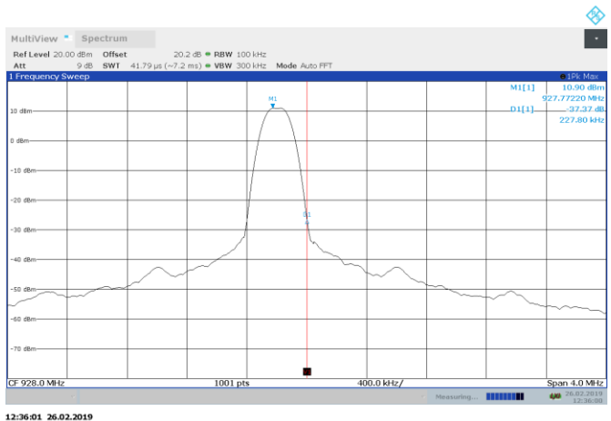
Figure 8.7-14: Conducted spurious emissions at the upper band edge, High channel
