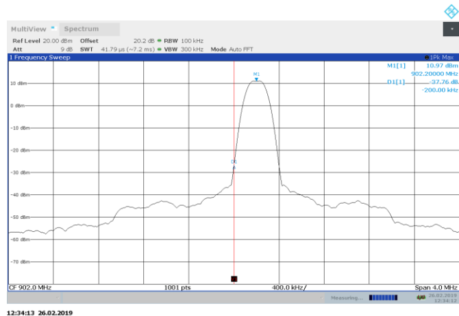
Figure 8.7-13: Conducted spurious emissions at the lower band edge, Low channel
