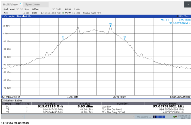
Figure 8.5-5: 99% OBW on mid channel
