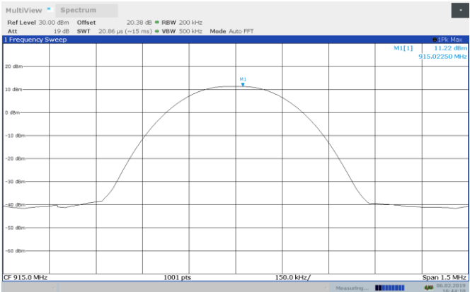
Figure 8.6-2: Peak output power on mid channel
