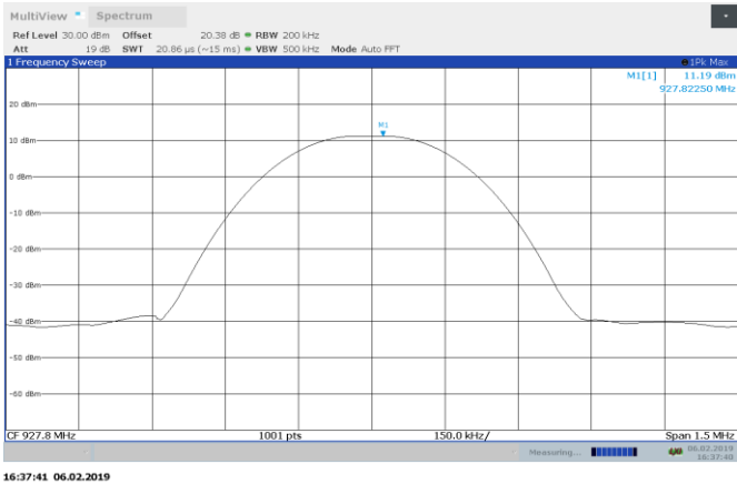
Figure 8.6-3: Peak output power on high channel
