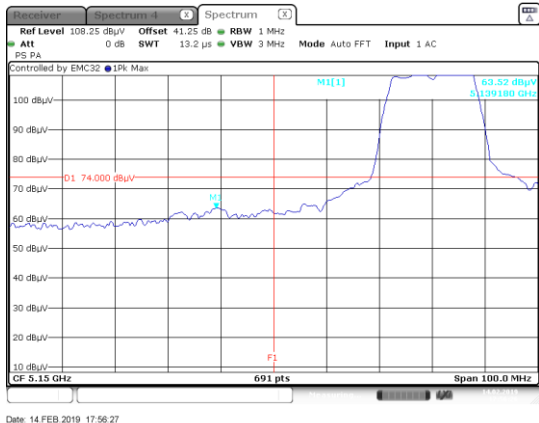
Figure 8.8-1: Radiated – Undesirable (unwanted) emissions within restricted band at 5.15 GHz, Peak (Channel 36, 802.11a)
