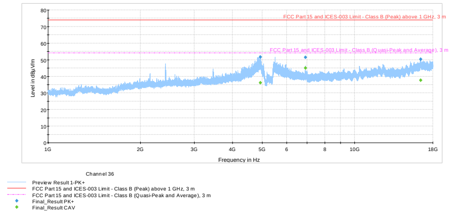
Figure 8.8-10: Radiated – Undesirable (unwanted) emissions 1 to 18 GHz, Channel 36 – 5180 MHz 802.11a
