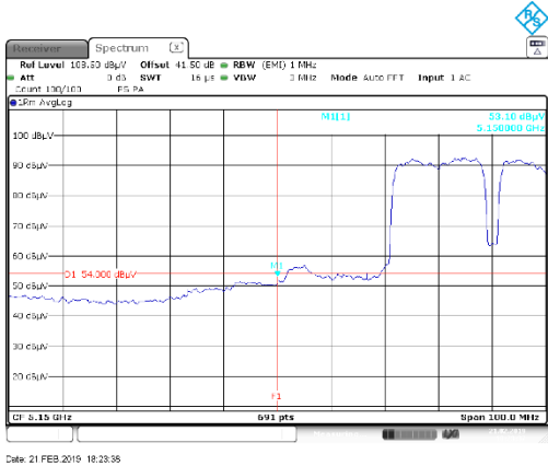
Figure 8.8-4: Radiated – Undesirable (unwanted) emissions within restricted band at 5.15 GHz, Average (Channel 36, 802.11n)
