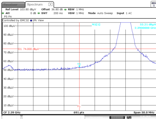
Figure 8.7-8: Radiated restricted bands spurious emissions at 2.39 GHz , peak
