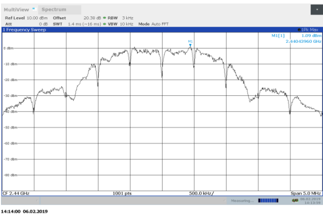
Figure 8.8-2: PSD sample plot on mid channel
