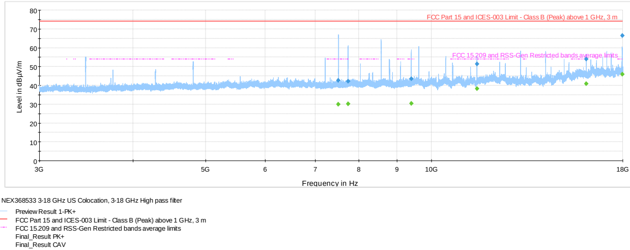
Figure 8.1-4: Radiated spurious emissions products from co-located transmitters within 3–18 GHz
