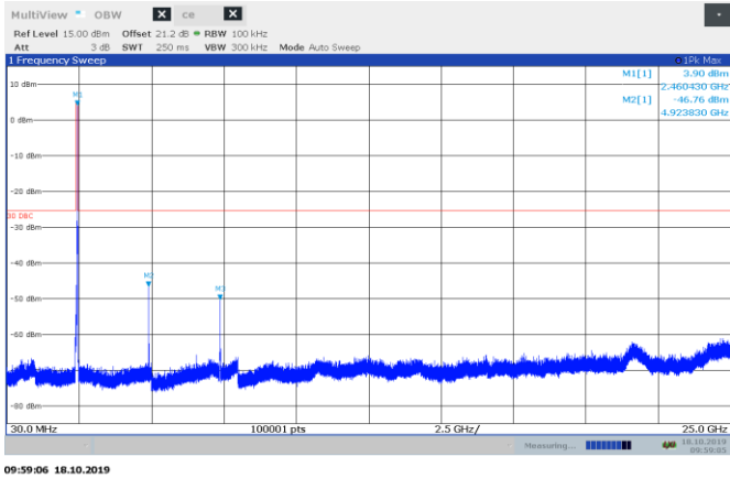
Figure 8.7-69: Conducted spurious emissions for 802.11b, high channel
