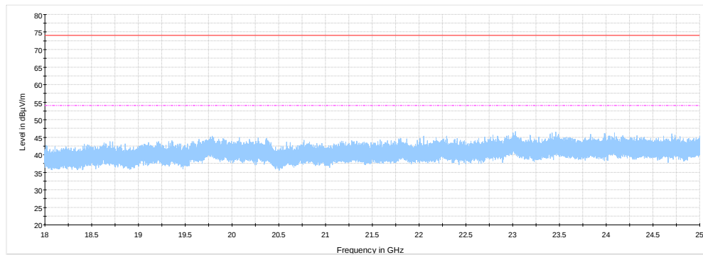
Figure 8.7-50: Radiated spurious emissions 18 - 25 GHz for 802.11n HT40, low channel
