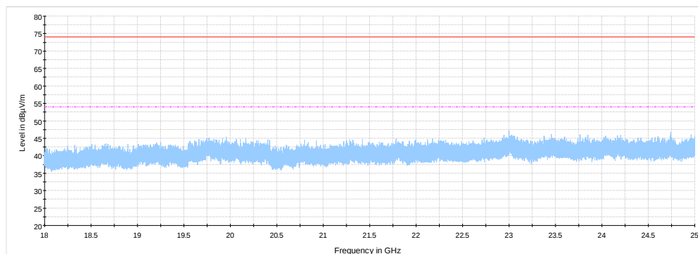
Figure 8.7-51: Radiated spurious emissions 18 - 25 GHz for 802.11n HT40, mid channel
