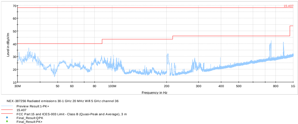
Figure 8.7-5: Radiated – Undesirable (unwanted) emissions 30 MHz - 1 GHz, Channel 36 – 5180 MHz, 802.11a
