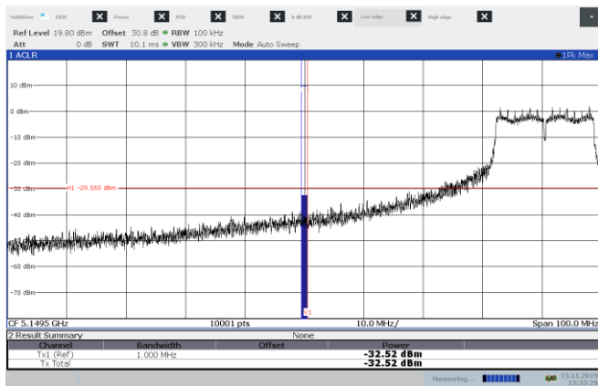
Figure 8.7-20: Conducted band edge emissions at 5.15 GHz, (Channel 36, 802.11a)
