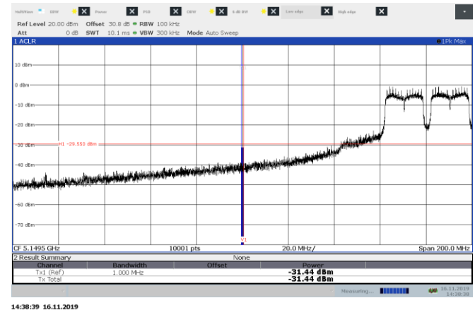
Figure 8.7-23: Conducted band edge emissions at 5.15 GHz, (Channel 48, 802.11n)
