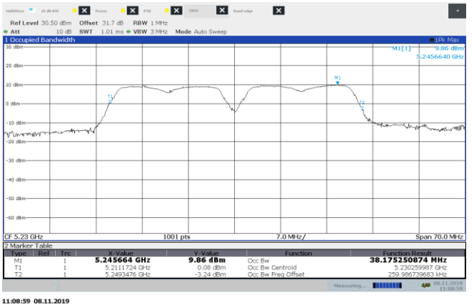
Figure 8.5-4: 99 % bandwidth on 802.11n, sample plot
