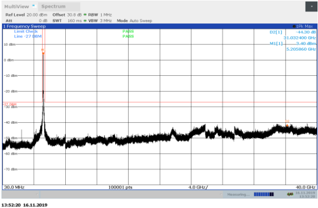
Figure 8.7-27: Conducted spurious emissions 30 MHz – 40 GHz, Channel 36 – 5190 MHz, 802.11n
