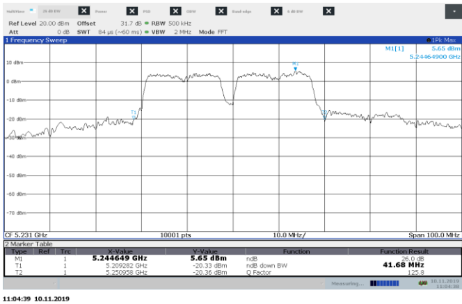
Figure 8.5-2: 26 dB bandwidth on 802.11n, sample plot
