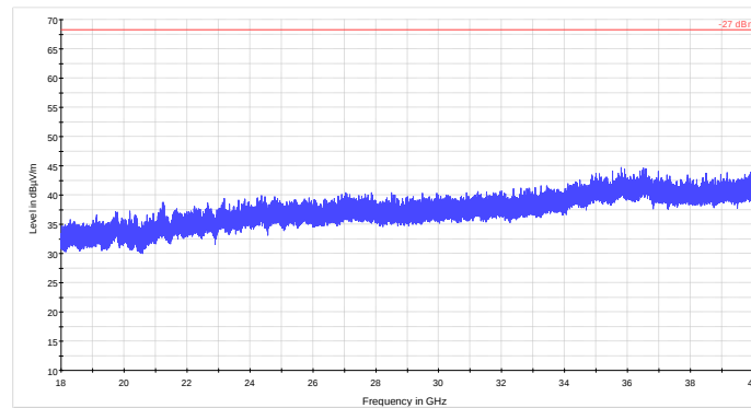
Figure 8.7-18: Radiated spurious emissions 18 - 40 GHz low channel, 802.11n
