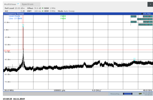
Figure 8.7-28: Conducted spurious emissions 30 MHz – 40 GHz high channel, 802.11n
