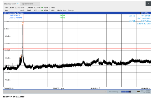
Figure 8.7-27: Conducted spurious emissions 30 MHz – 40 GHz low channel, 802.11n
