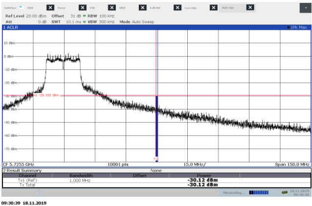
Figure 8.7-28: Conducted band edge emissions 5.725 GHz, channel 136, 802.11a
