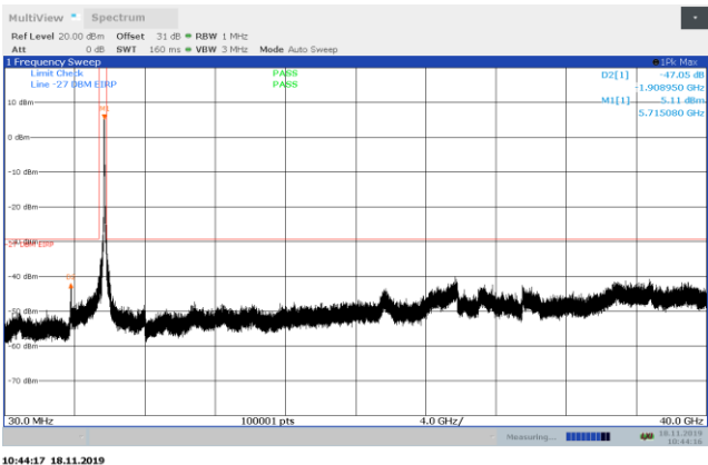
Figure 8.7-34: Conducted spurious emissions 30 MHz – 40 GHz, high channel, 802.11a
