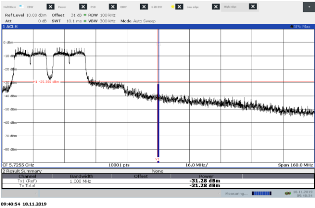
Figure 8.7-29: Conducted band edge emissions 5.725 GHz, channel 136, 802.11n
