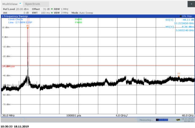
Figure 8.7-32: Conducted spurious emissions 30 MHz – 40 GHz, low channel, 802.11a
