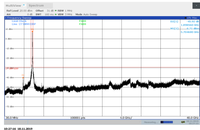
Figure 8.7-37: Conducted spurious emissions 30 MHz – 40 GHz, high channel, 802.11n
