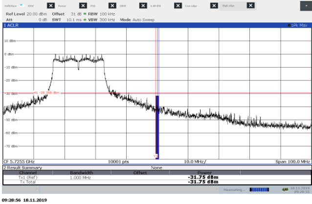
Figure 8.7-27: Conducted band edge emissions 5.725 GHz, channel 140, 802.11a
