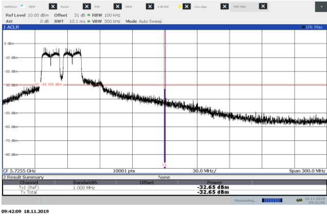
Figure 8.7-30: Conducted band edge emissions 5.725 GHz, channel 132, 802.11n
