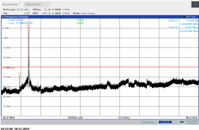
Figure 8.7-33: Conducted spurious emissions 30 MHz – 40 GHz, mid channel, 802.11a
