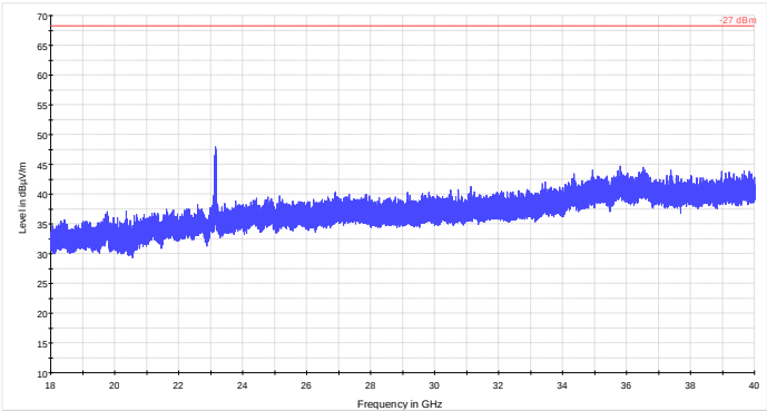
Figure 8.8-11: Radiated spurious emissions 18 - 40 GHz low channel, 802.11a
