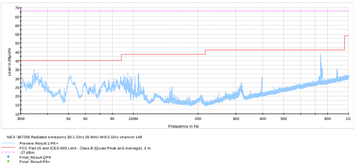
Figure 8.8-4: Radiated spurious emissions 30 MHz – 1 GHz low channel, 802.11n
