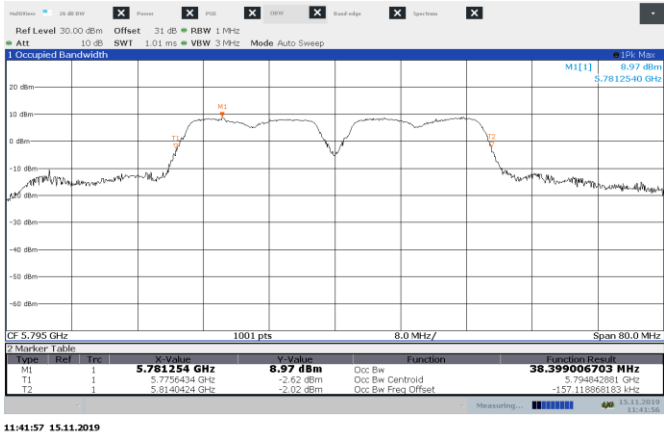
Figure 8.6-4: 99 % bandwidth on 802.11n, sample plot
