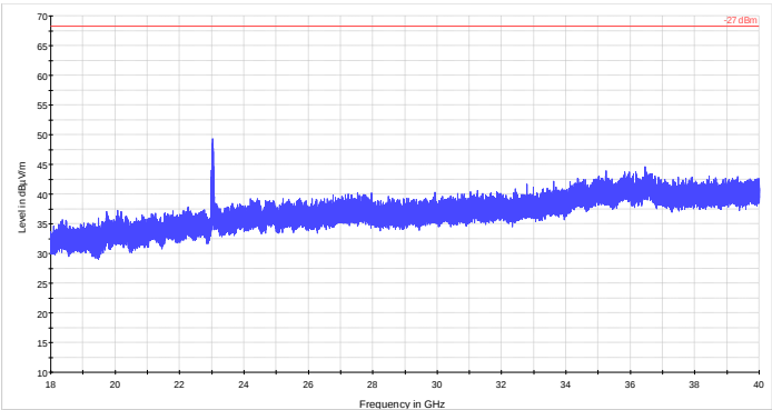
Figure 8.8-14: Radiated spurious emissions 18 - 40 GHz low channel, 802.11n
