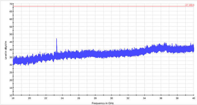
Figure 8.8-12: Radiated spurious emissions 18 - 40 GHz mid channel, 802.11a
