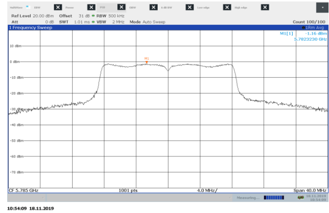
Figure 8.7-3: Sample plot for PSD on 802.11a
