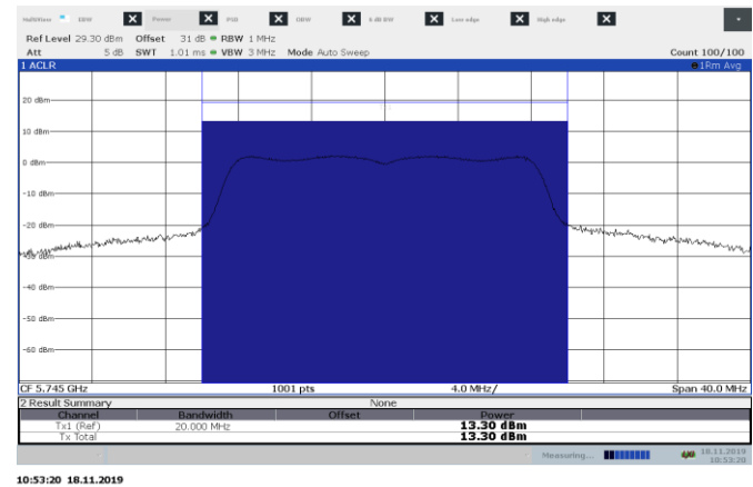
Figure 8.7-1: Sample plot for Power on 802.11a
