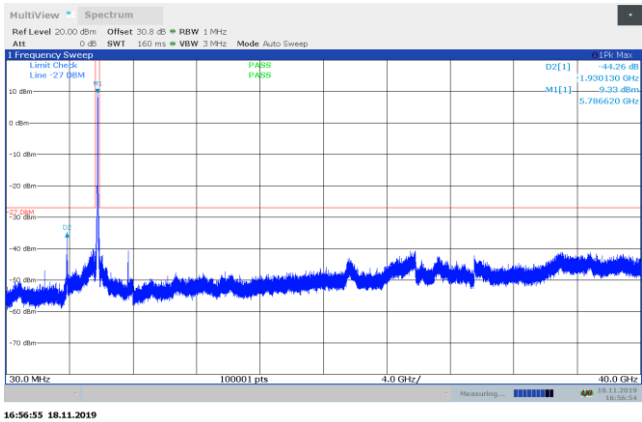
Figure 8.8-21: Conducted spurious emissions 30 MHz – 40 GHz mid channel, 802.11a
