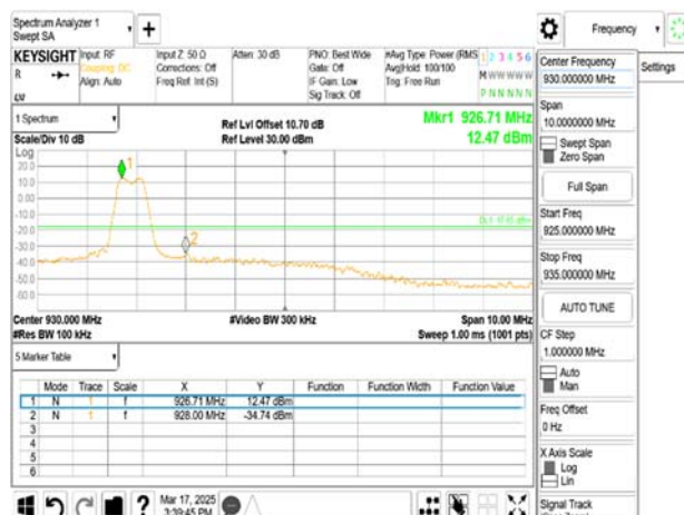
Band Edge_FSK_100Kbps_HighCH-926.9MHz
