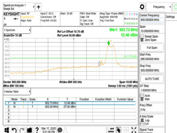
Band Edge_FSK_100Kbps_LowCH-902.9MHz
