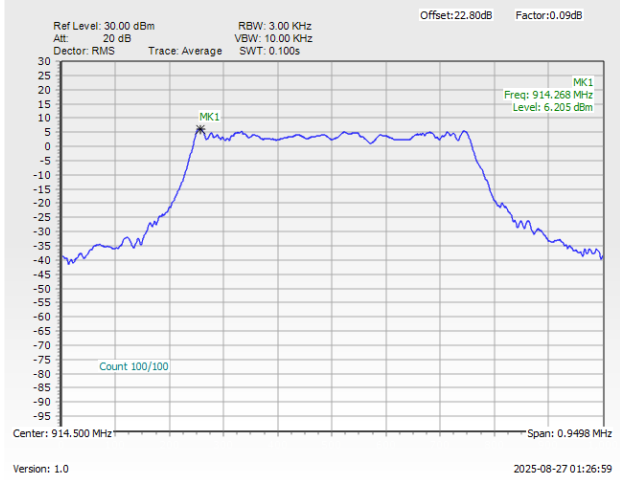
Power Density (dBm/3kHz) Plot Channel 15
