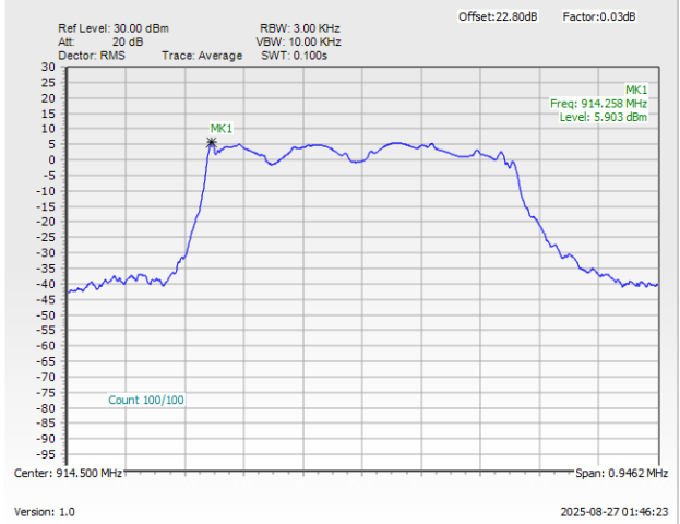
Power Density (dBm/3kHz) Plot Channel 15
