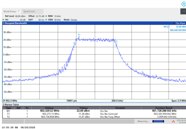
99% Occupied Bandwidth Plot on Channel 30
