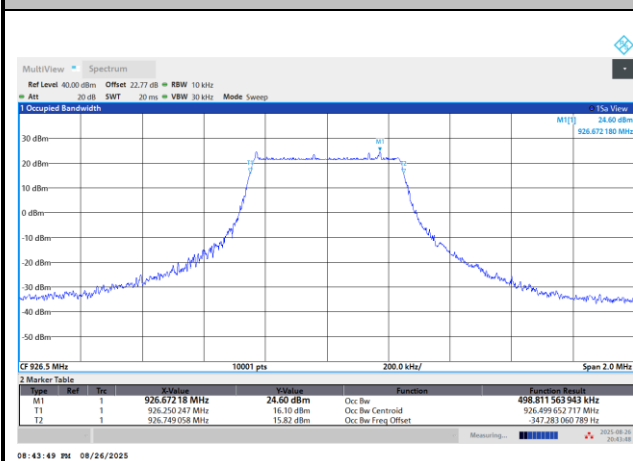
99% Occupied Bandwidth Plot on Channel 30
