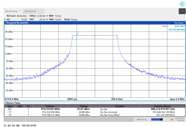
99% Occupied Bandwidth Plot on Channel 15
