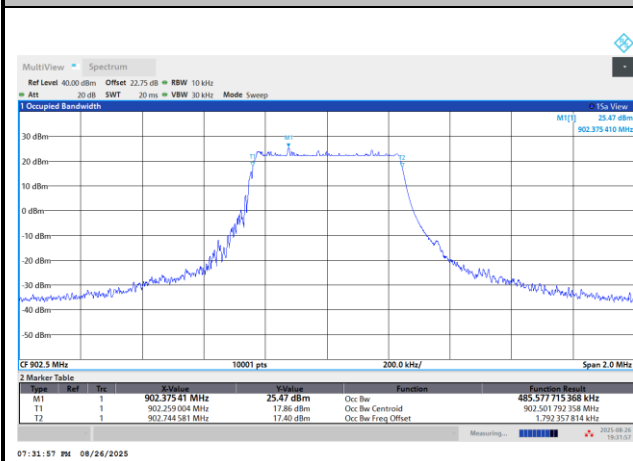
99% Occupied Bandwidth Plot on Channel 0
