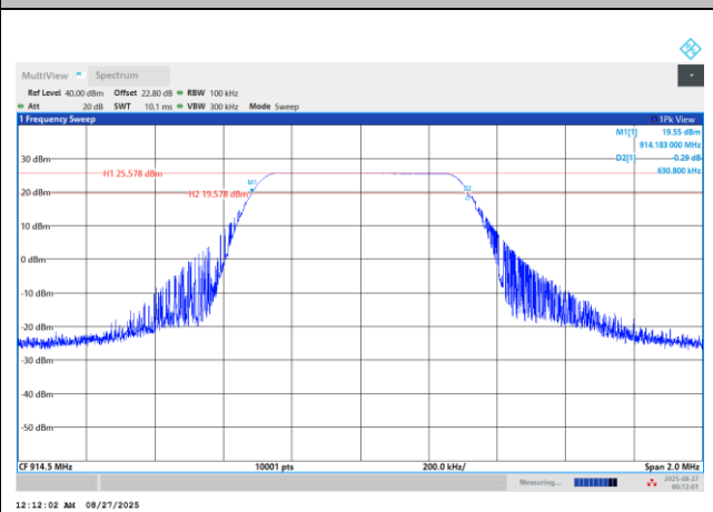
6 dB Bandwidth Plot on Channel 15
