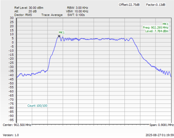
Power Density (dBm/3kHz) Plot Channel 30
