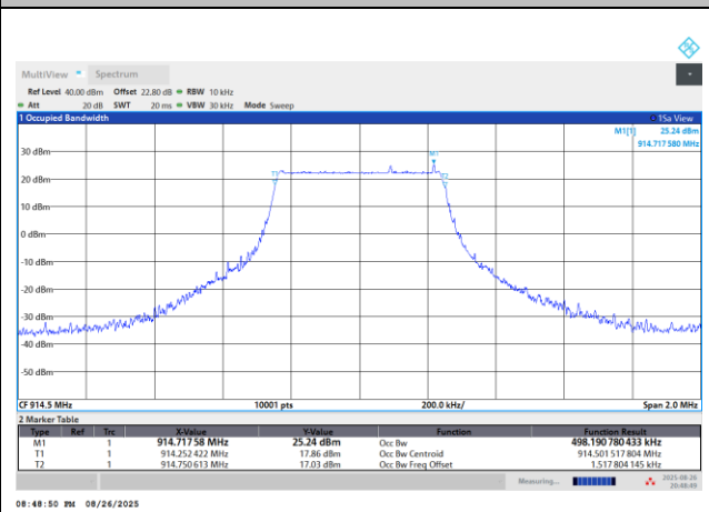
99% Occupied Bandwidth Plot on Channel 15
