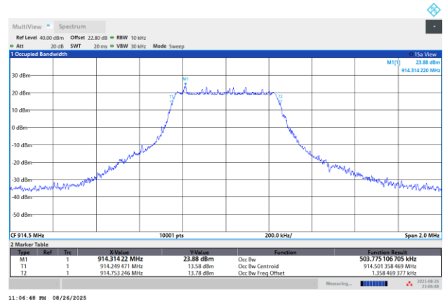
99% Occupied Bandwidth Plot on Channel 15
