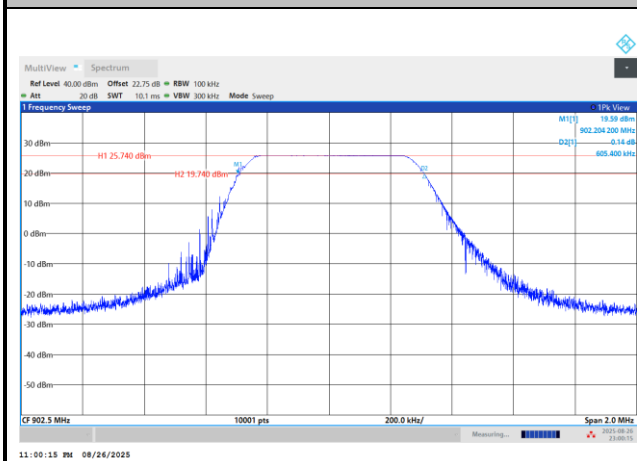
6 dB Bandwidth Plot on Channel 0
