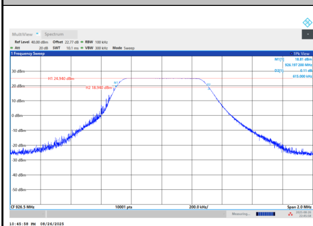
6 dB Bandwidth Plot on Channel 30
