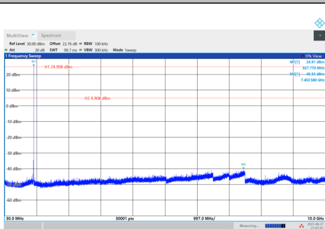
CSE Plot on High Ch between 927.8MHz
