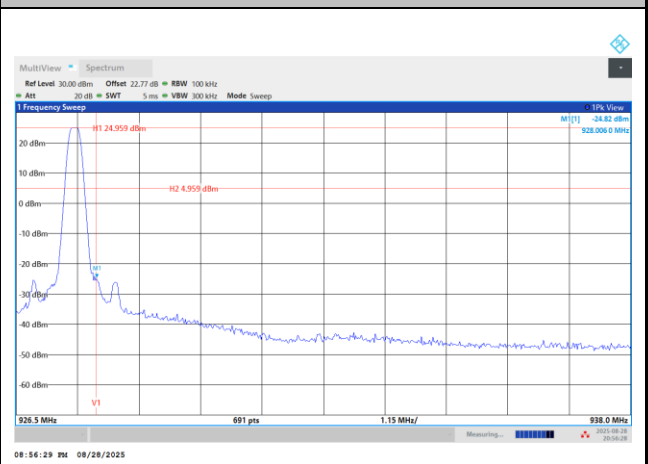
High Band Edge Plot on 927.6MHz
