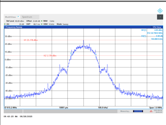
20 dB Bandwidth Plot in 915.2MHz
