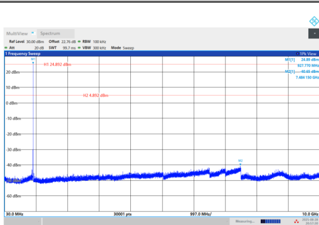
CSE Plot on High Ch between 927.6MHz
