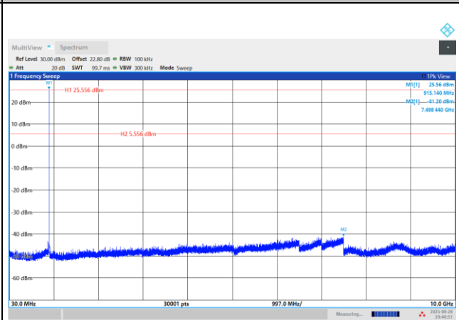
CSE Plot on Mid Ch between 915.2MHz
