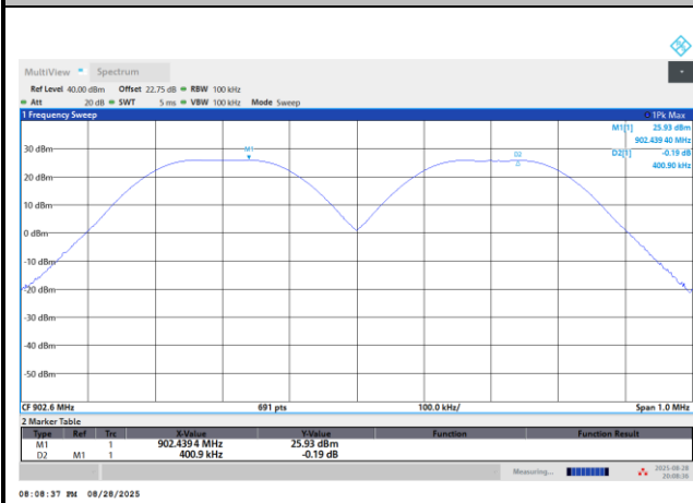
Channel Separation Plot on 902.4MHz
