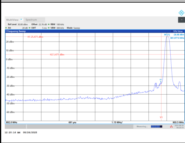
Low Band Edge Plot on 902.4MHz
