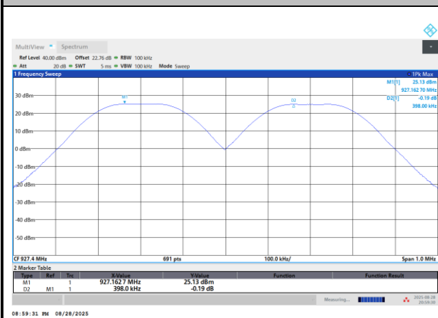
Channel Separation Plot on Channel 927.6MHz
