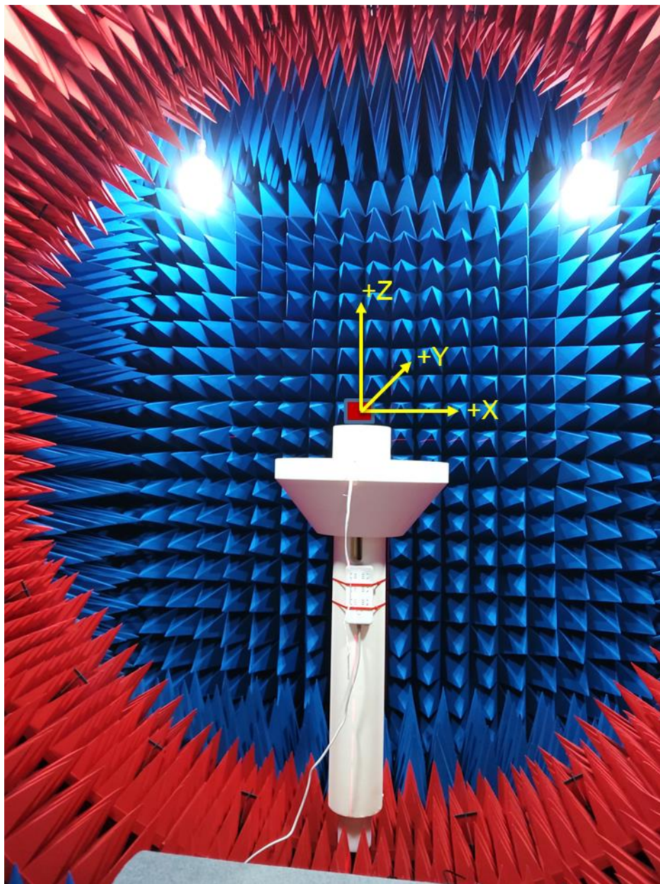
Setup photograph:
