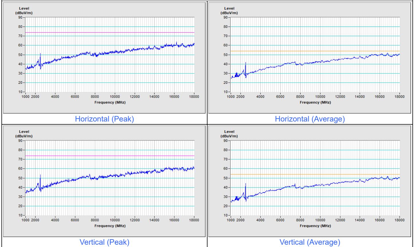
BT LE-2M Channel 39
