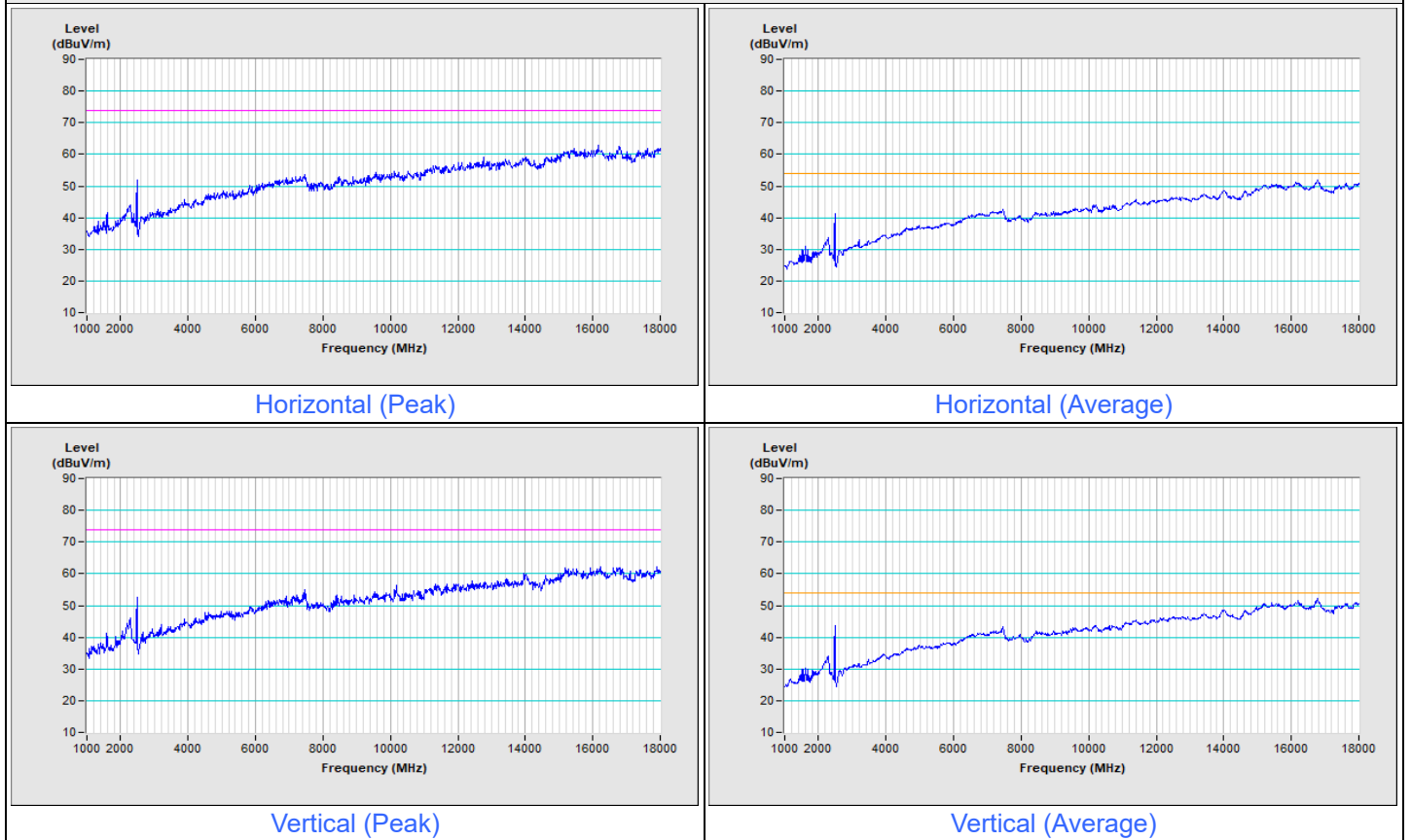
BT LE-125K Channel 39
