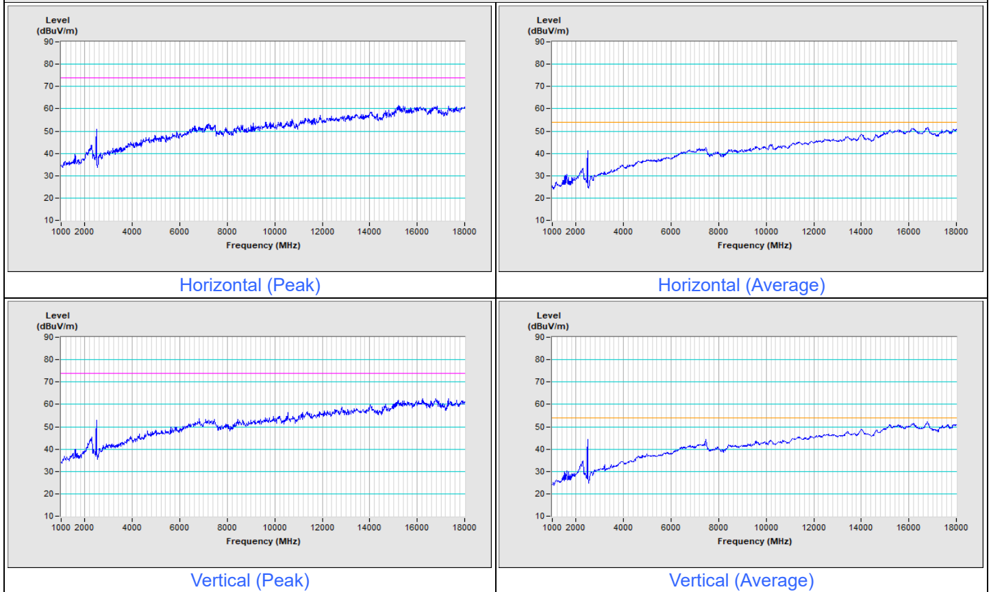
BT LE-500K Channel 39
