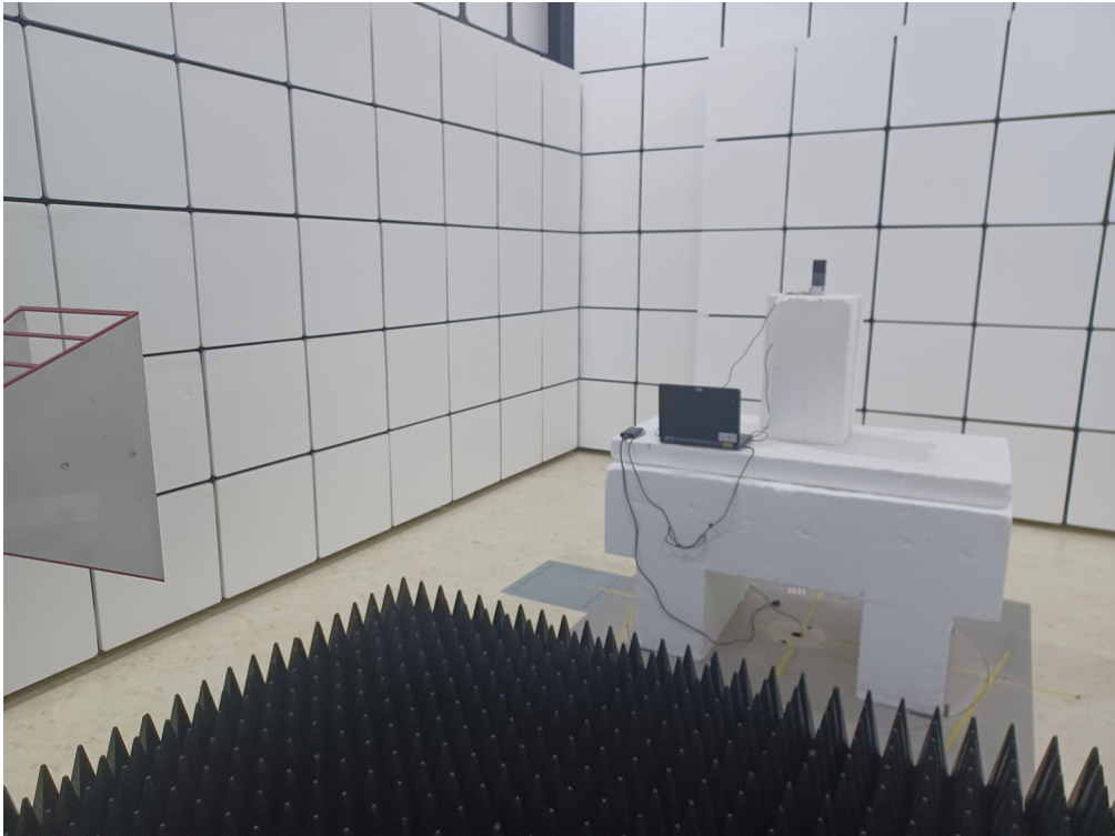
Radiated Test (18 -40 GHz)
