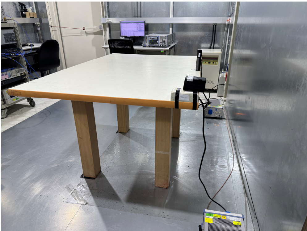
Back View of AC Power Line Conducted Emission Test AC Adapter (AD-2410)
