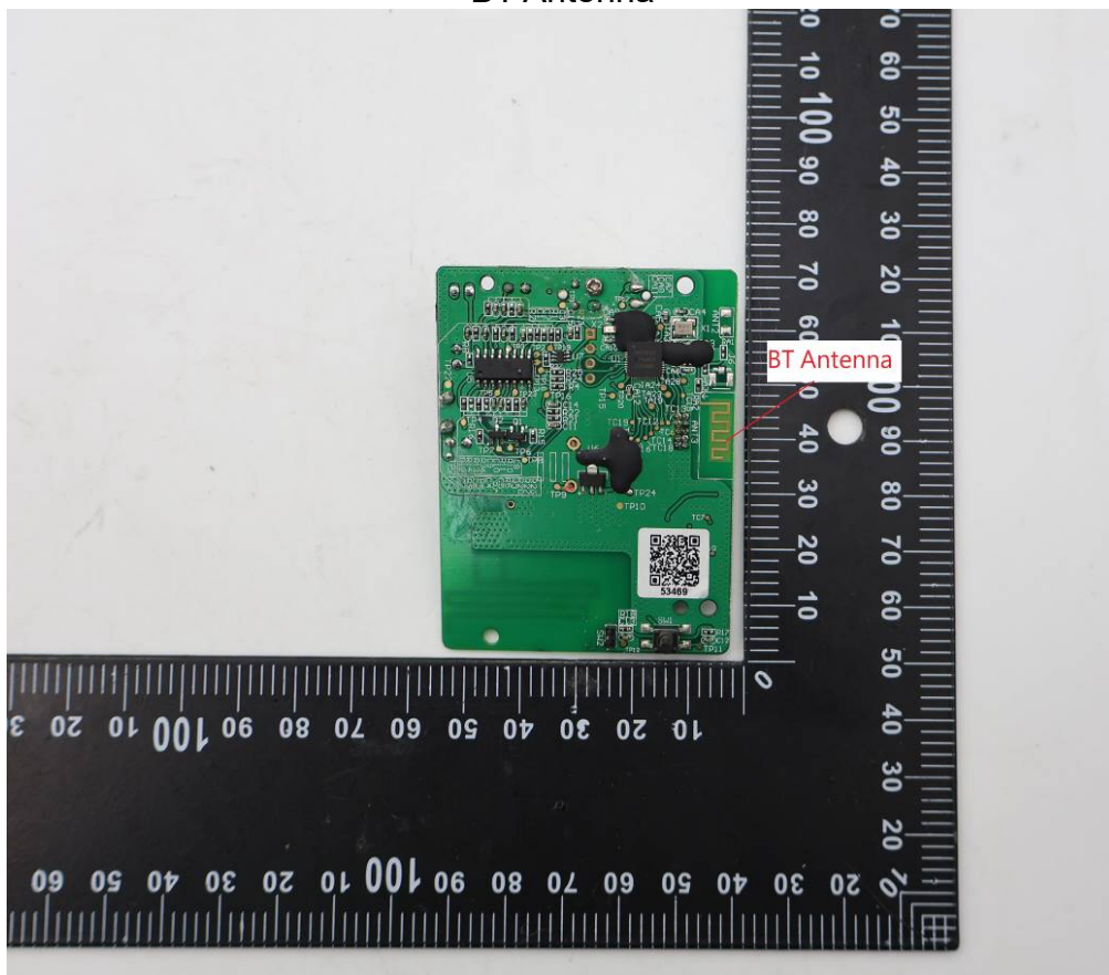
BT Antenna
