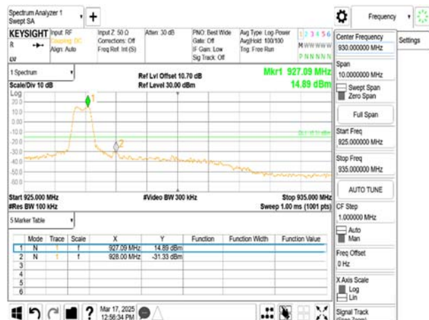
Band Edge_FSK_100Kbps_HighCH-926.9MHz
