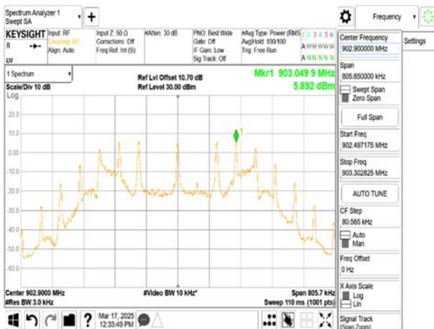
PSD_FSK_100Kbps_LowCH-902.9MHz
