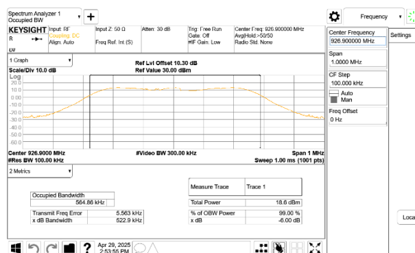
OBW_FSK 100Kbps 249bytes_HighCH-926.9MHz
