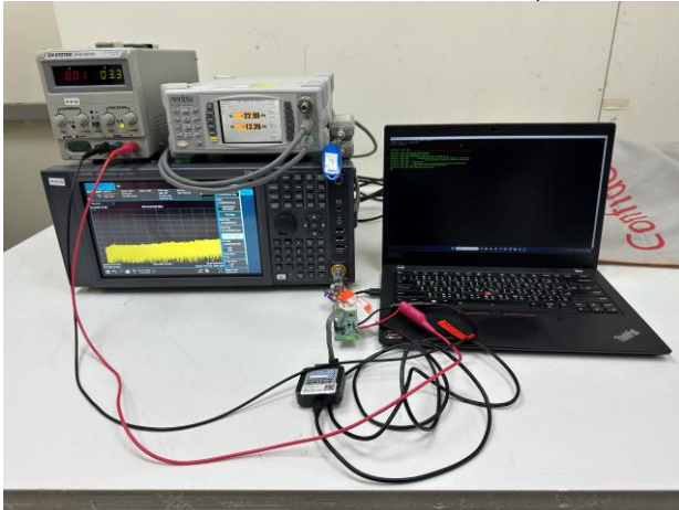
FCC_15_247_900MHz_Radiated_Setup
