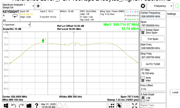
Reference Level_FSK 100Kbps 249bytes_HighCH-926.9MHz
