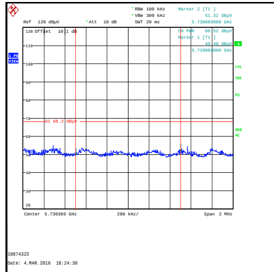
Upper Band Edge Measurement Integration method (emission at 5730.369 MHz)
