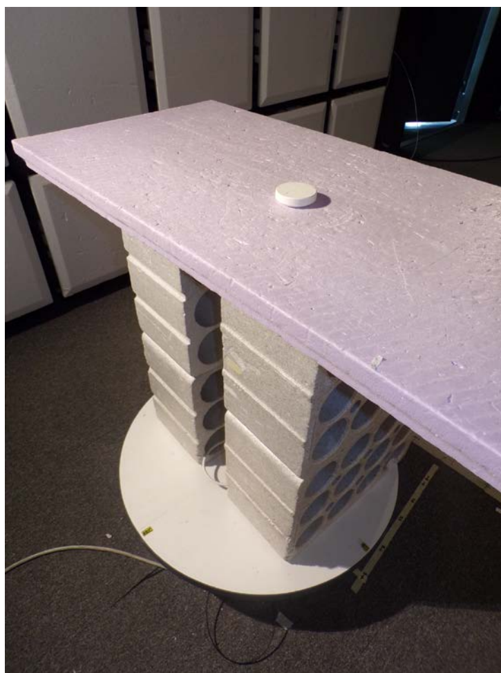
Radiated emission below 1GHz
