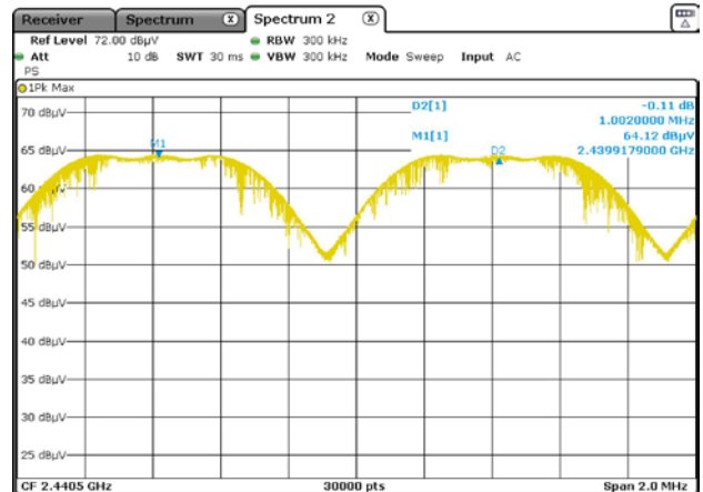
Channel separation
