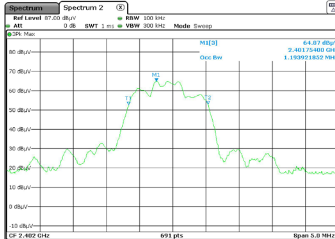
Low channel
