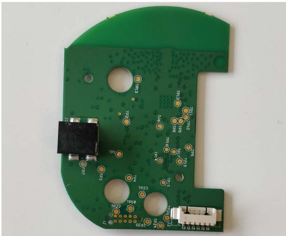
Charging base PCB
