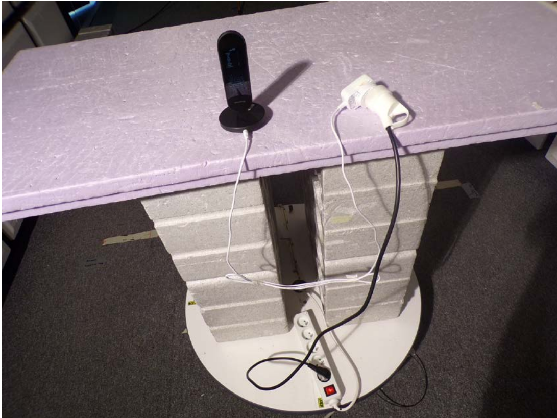
Test setup for radiated emission below 1GHz
