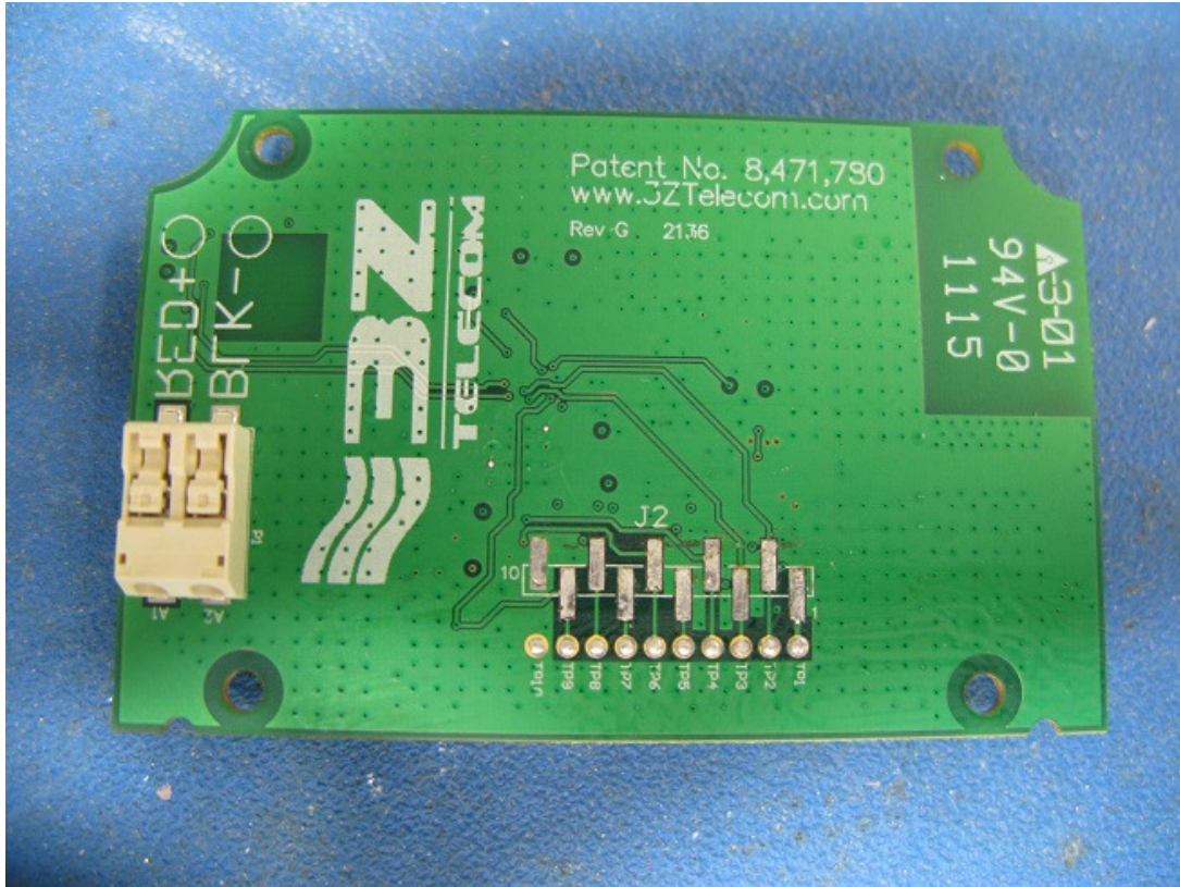
WASP Sensor Board (bottom)
