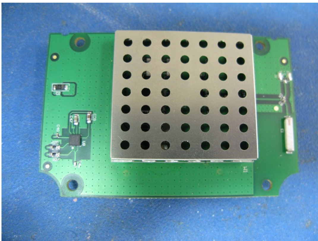
WASP Sensor Board with RF shield installed (top)
