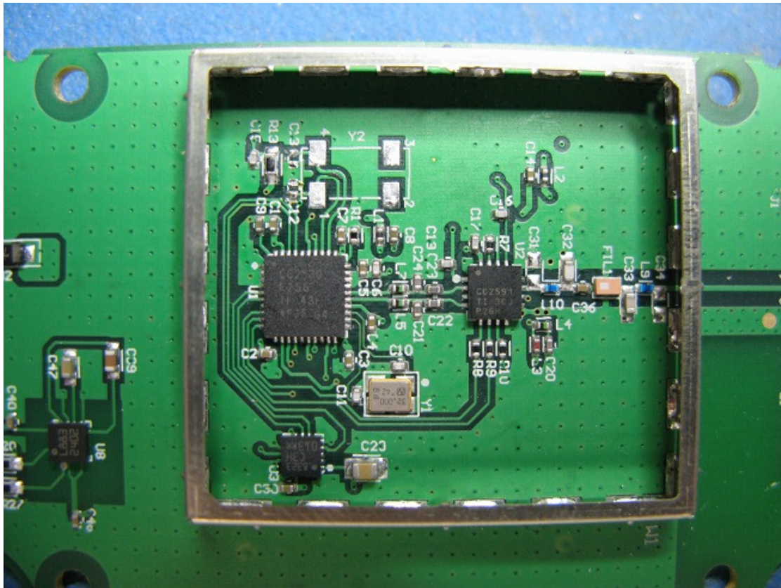
WASP Sensor Board with RF shield removed (top)
