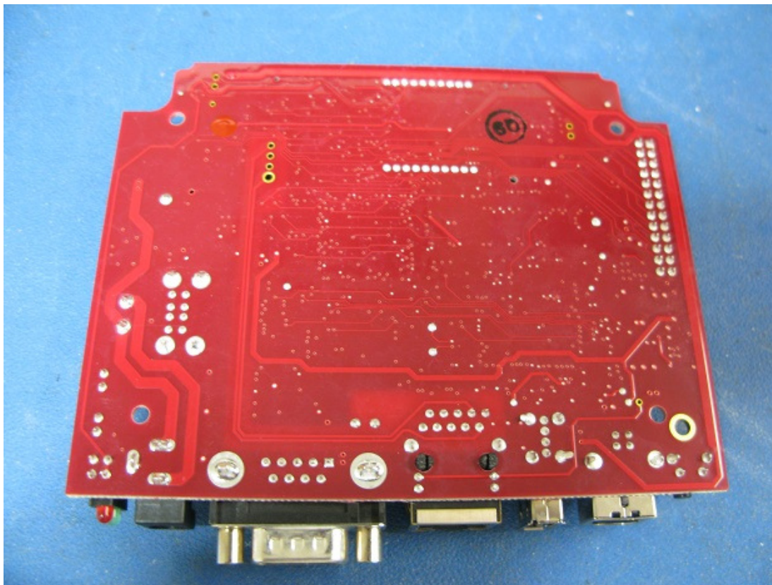
Single Board Computer (bottom)
