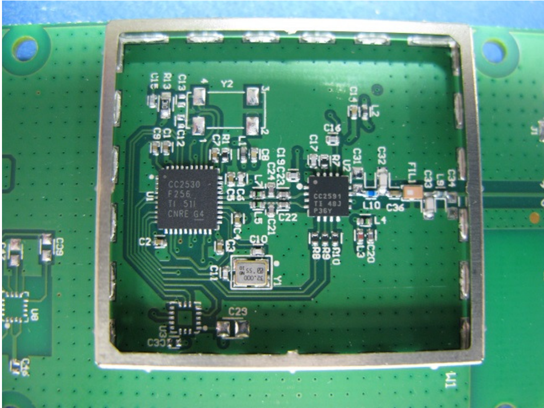
2.4GHz Radio Board with RF shield removed (top)
