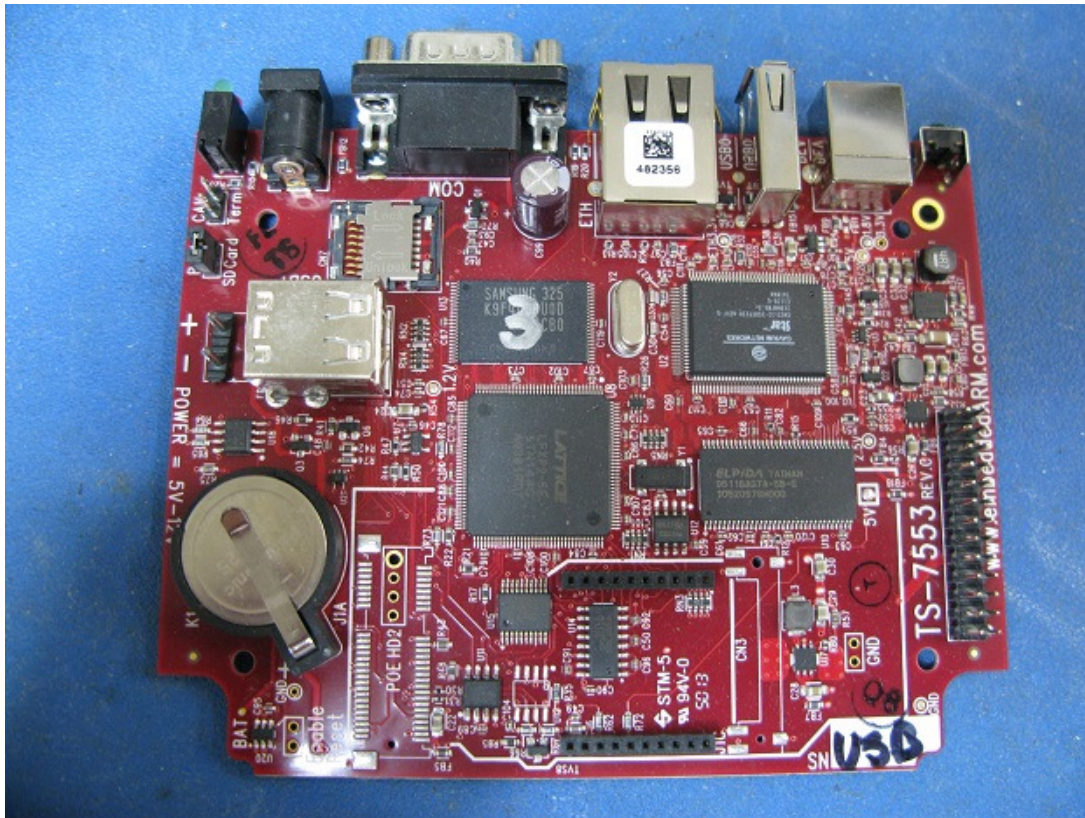
Single Board Computer (top)
