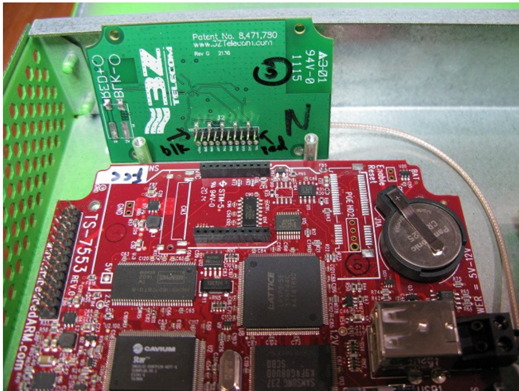
2.4GHz Radio Board unplugged from Single Board Computer
