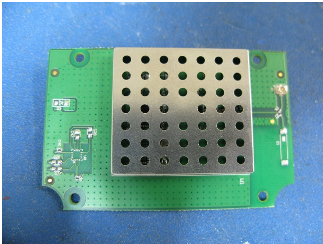
2.4GHz Radio Board with RF shield installed (top)
