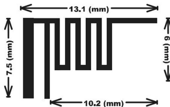
Antenna design
