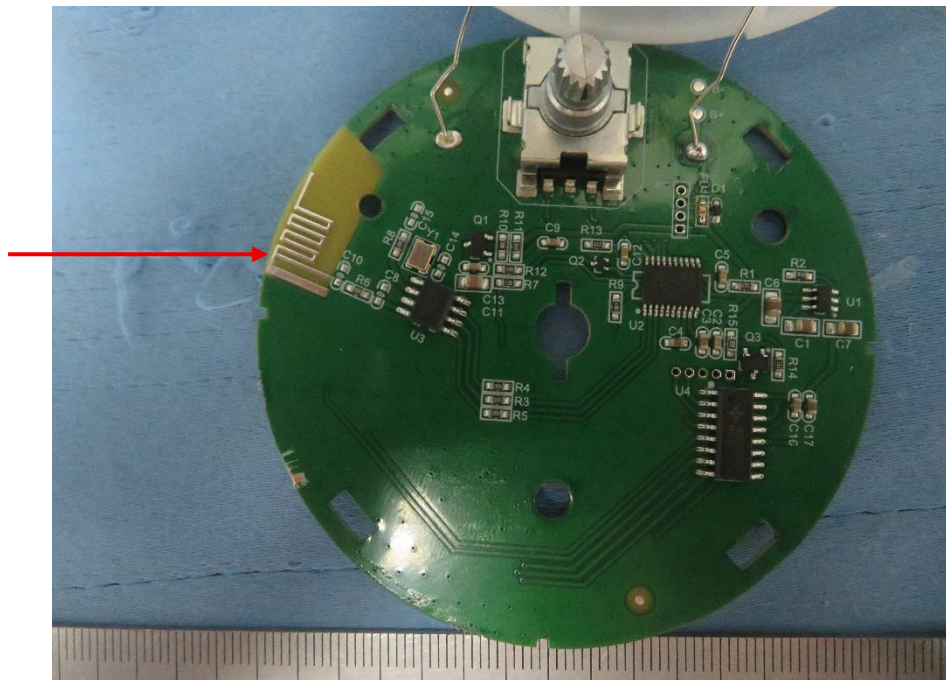
Antenna design
